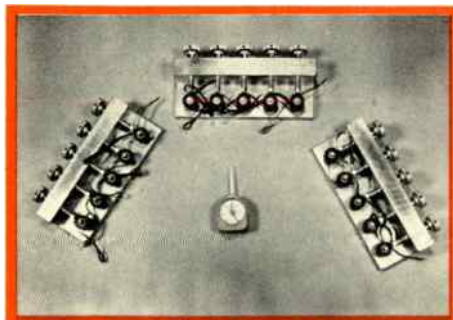
Test fixtures to check rollers for tape-stick.
