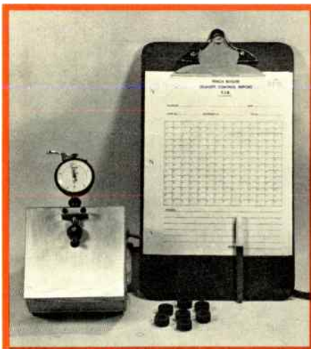
Gauges developed for TIR in increments of .00025.
