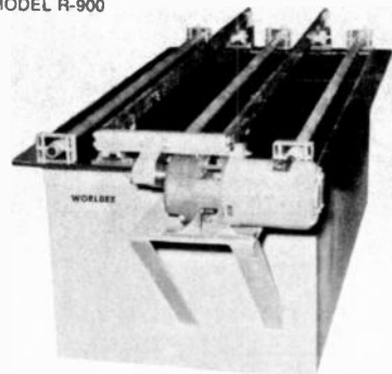
12-POSITION PLATING TANK 1/8" SEAMLESS LINING OVER STEEL, WITH OVERFLOW TANK MODEL PL64-12
