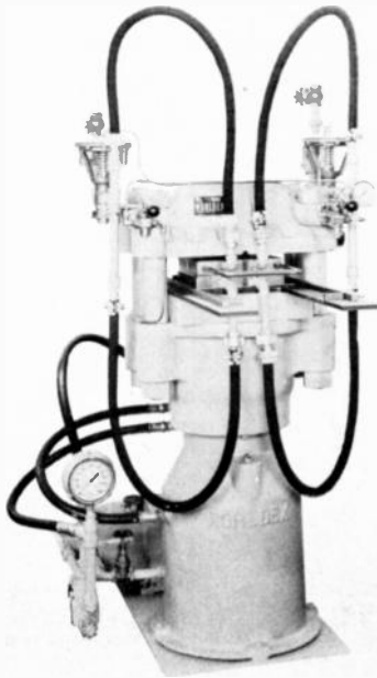
HYDRAULIC RECORD PRESS MODEL W-1246A
