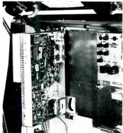
SWING-OUT COMPONENTS
