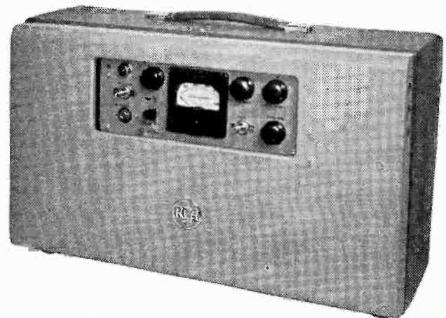
THE RELAY RECEIVER consists of the receiver unit itself, which is mounted on the rear of a parabolic reflector (and is similar in appearance to the transmitter unit) plus the receiver control unit shown above. The parabolic and receiver can be mounted on a permanent structure as shown at the top of this page or on a tripod similar to that used with the transmitter. The control unit is assembled on a bathtub-type chassis (top) which can be mounted on a standard rack or in a portable carrying case (bottom).
