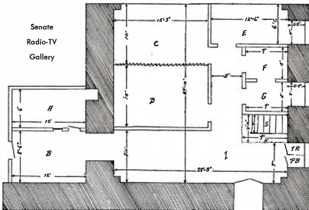
THIS SKETCH shows preliminary plans for the $33,000 remodeling of the Senate Radio-TV Gallery. Architect plans already have been drawn and construction begun. Subcontracts have not yet been let [B•T, Aug. 31]. Legend: A—present TV studio to be used as radio studio, 12 x 6 ft.; B—outer office 12 x 8½ ft.; C and D—make up new TV studio, 20 x 15¼ ft., will have acoustical doors permitting two studios, 10 x 15¼ ft., which can be used for filming of two separate shows at the same time; E—radio studio, 12½ x 6½ ft.; F—radio studio, 7 x 5 ft.; G—radio studio, 7 x 5 ft. (F and G can be combined by opening acoustical door giving 10 x 7 ft. space for radio); H—stairs leading to mezzanine (17 x 12½ ft.) for use of files, power, telephones and air conditioning controls; I—office space 28¼ x 8 ft. 10 inches. (TR is teletype room, PB is phone booth.) Lines will be included for any of the networks (radio and TV) to use studios. Acoustical tile and grid lighting are among many modern installations planned. Target month for completion is next January. Capitol workmen are being used.
