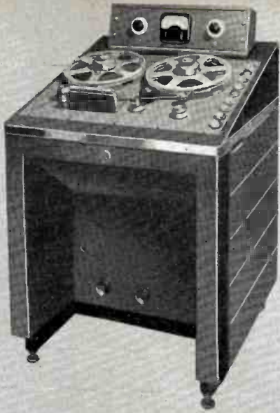
RT-12B PROFESSIONAL TAPE RECORDER (CONSOLE TYPE). Same as RT-11B and includes all the design features of the rack-mounted unit—but is ideal for use near the RCA Consolette or turntables in control rooms or studios where rack space is not available.
