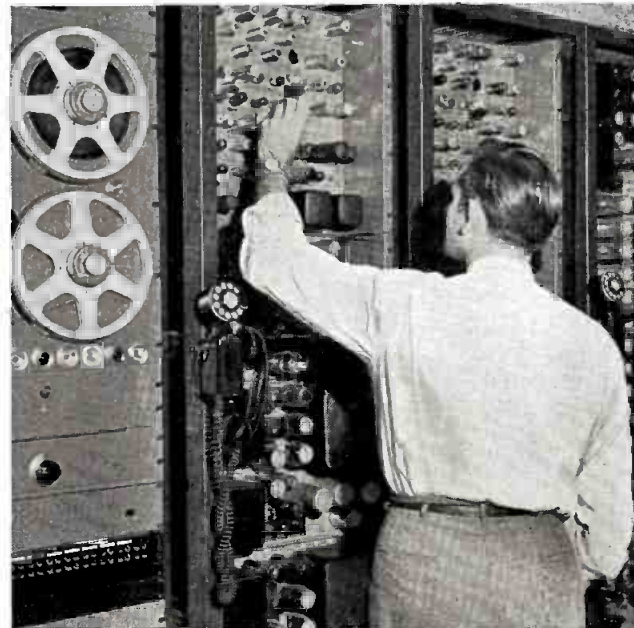
SIMPLE RACK ADDITIONS! Closeup of the two cabinet racks containing auxiliary and power equipment for the two vidicon film cameras. Only the vidicon control chassis and vidicon deflection chassis (top and next to top panels in each rack) had to be installed in each chain. Power supplies were already part of original equipment. Racks are readily accessible for setup, adjustment and maintenance.
