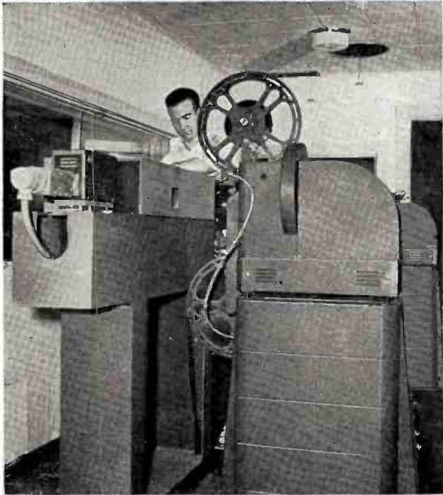
TWO FILM CHAINS MODIFIED! Picture above shows modernized WAAM-TV film projection room. The RCA TK-21 Vidicon Cameras are mounted on TP-11 Multiplexers. One TP-16 Film Projector, one 35 mm slide projector and an opaque projector are used with each camera. The two independently operated chains increase ease of operation and provide preview and auditioning facilities.
