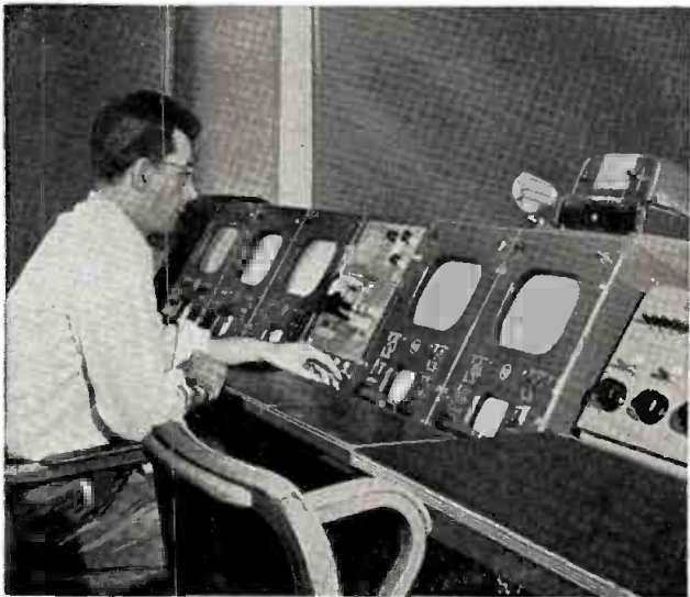
MINOR CHANGES IN CONTROL ROOM! Second and third monitors from left are the vidicon master monitors. Their housings also enclose the camera control panels. Installation was relatively simple since the station's original film monitors and housings were used. No changes in arrangement were required—vidicon control panels being substituted for control panels of the iconoscope cameras.
