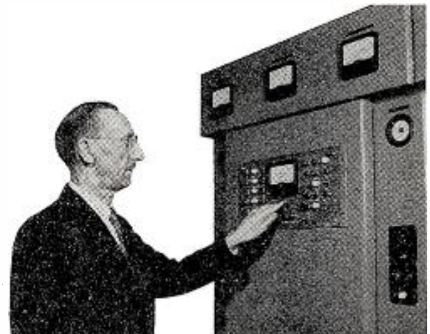
Andrew Friedenthal at Continental's Type TRC remote control panel . . . built into the Type 317B 50 KW transmitter.
