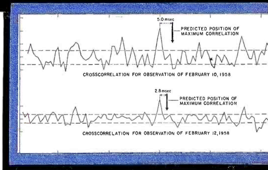
Correlation curves showing radar returns from Venus. The central peaks indicate the exact time of the radar waves from Earth to Venus and back (about five minutes). Each peak is the result of elaborate calculations by a high-speed digital computer on many thousands of tiny echoes originally beamed by Continental Electronics' transmitter
