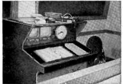
This Favag secondary, located in the announcer's console, has an oil bath movement for complete silence. Other secondaries are located in the Film Projection VTR room, the main studio, the Master Control room and in the news editing room.
