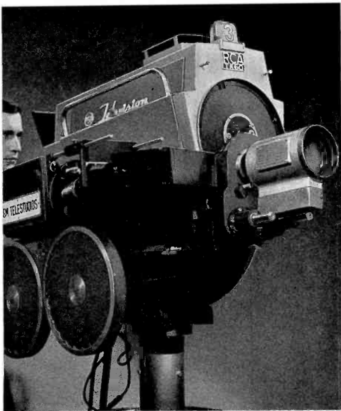
"GEMINI" —is the name of this twin camera system, employing a TK-60 Studio Camera which shares its lens with a 16mm film camera adjacently mounted. The operator uses the viewfinder of the television camera just as if he were shooting with the TK-60 alone. Final product, a high quality television tape and a high quality 16mm film duplicate, eliminates the problem of the kinescope as a factor in spot use of taped commercials and programs. Exclusive rights to "Gemini" are held by MGM.
