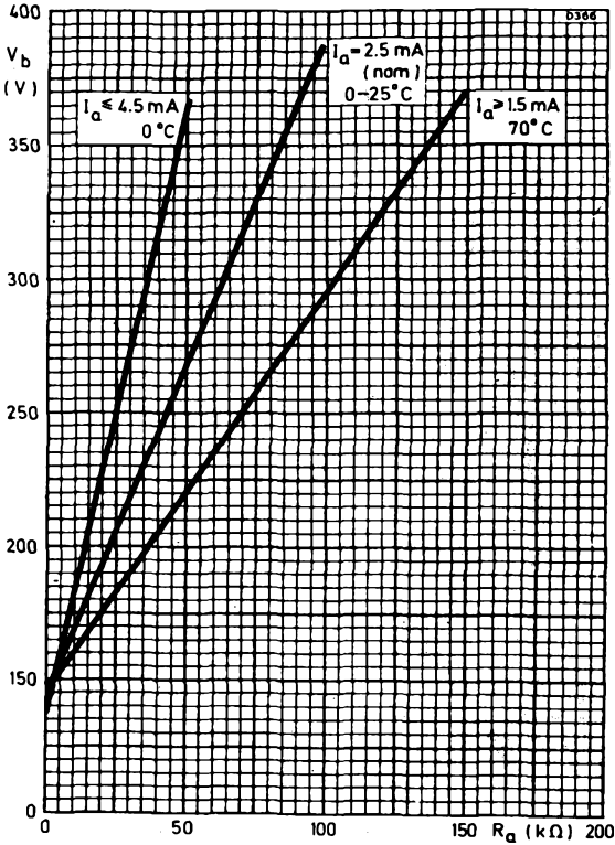
RELATIONSHIP BETWEEN D. C. SUPPLY VOLTAGE AND ANODE RESISTOR
