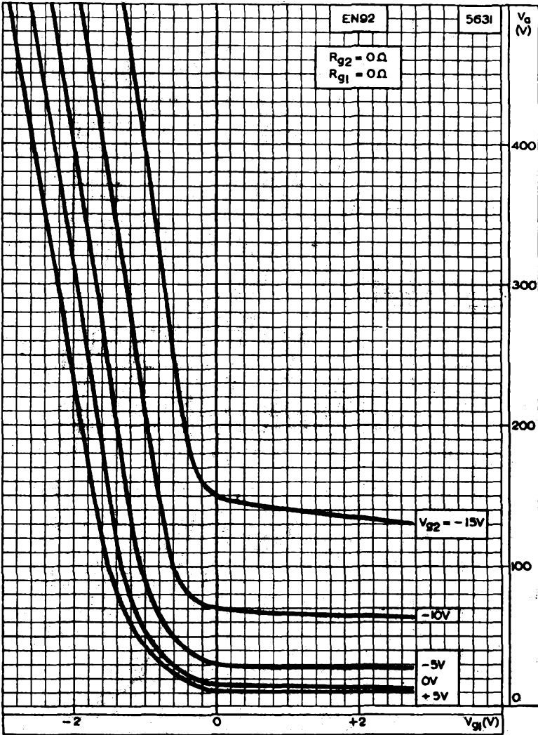
CONTROL CHARACTERISTICS
