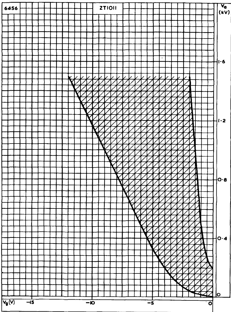
CONTROL CHARACTERISTIC
