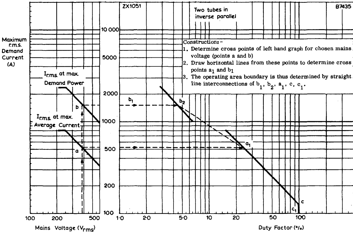
GRAPH RELATING DEMAND CURRENT WITH DUTY FACTOR AS A FUNCTION OF THE MAINS VOLTAGE. WELDING SERVICE ONLY
