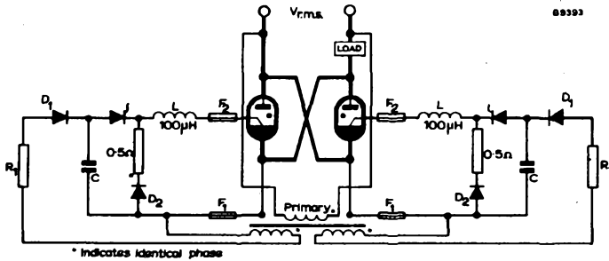
Figure 3:- Separate excitation
