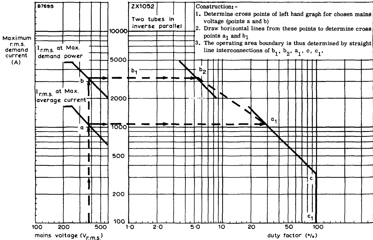
GRAPH RELATING DEMAND CURRENT WITH DUTY FACTOR AS A FUNCTION OF THE MAINS VOLTAGE, WELDING SERVICE ONLY
