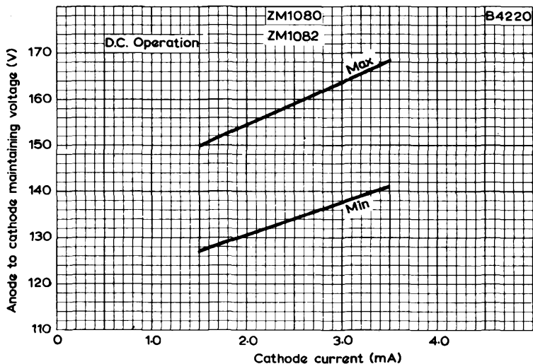
ANODE TO CATHODE MAINTAINING VOLTAGE PLOTTED AGAINST CATHODE CURRENT
