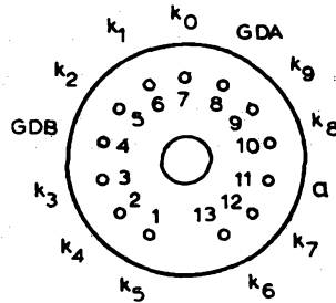
B13B Base
