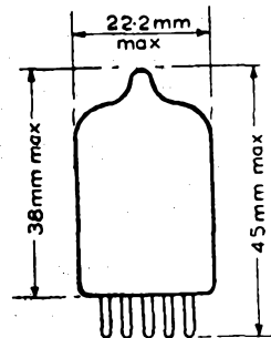
B9A Base
