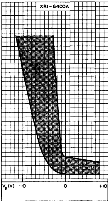
CONTROL CHARACTERISTIC
