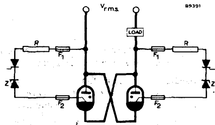
Fig.1: Anode excitation (Two thyristors)
