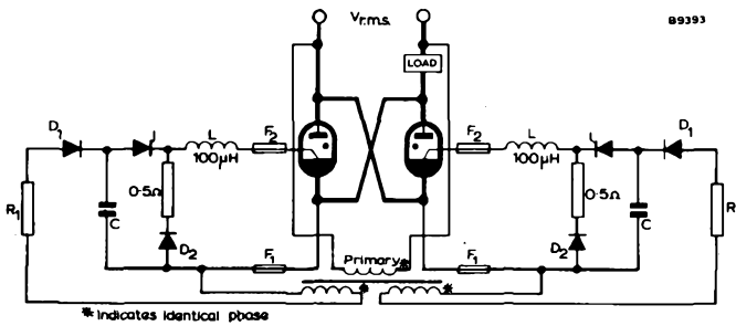
Figure 3:- Separate excitation
