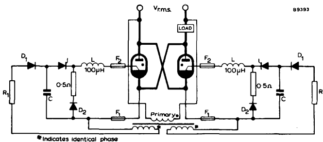
Fig. 3: Separate excitation
