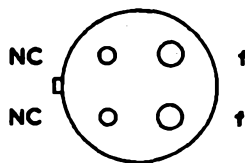
Medium 4-pin base with bayonet catch
