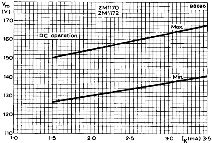
ANODE-TO-CATHODE MAINTAINING VOLTAGE PLOTTED AGAINST CATHODE CURRENT
