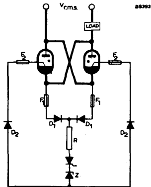
Figure 2:- Anode excitation (common thyristor)
