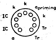
B9A Base
