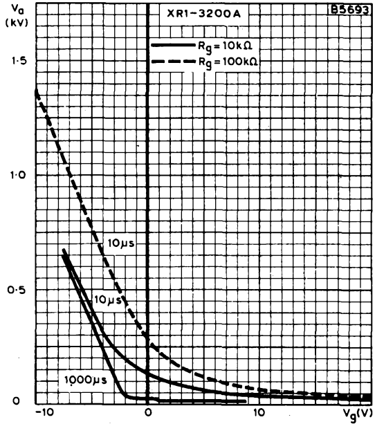
NOMINAL VARIATION BETWEEN ANODE AND GRID VOLTAGES FOR DIFFERENT IGNITION DELAY TIMES
