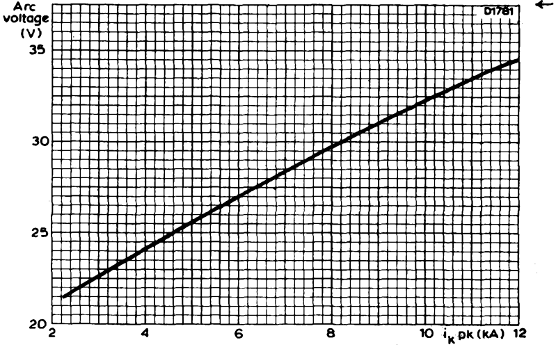
TYPICAL ARC VOLTAGE PLOTTED AGAINST CATHODE CURRENT
