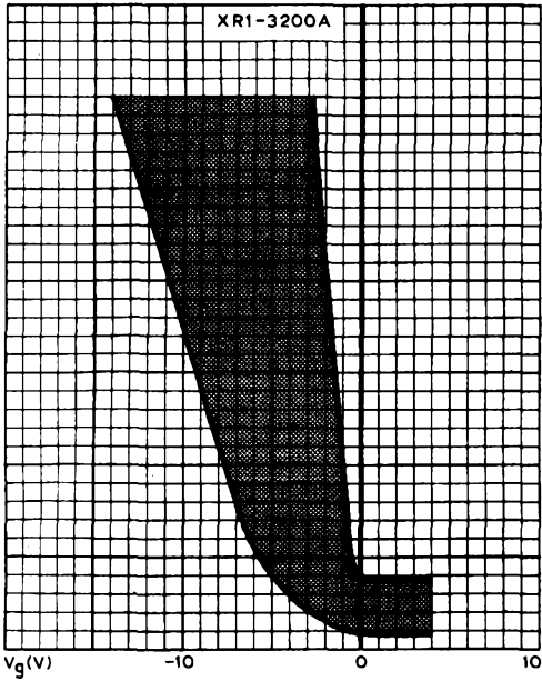
CONTROL CHARACTERISTIC
