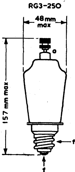
Medium Edison screw base
