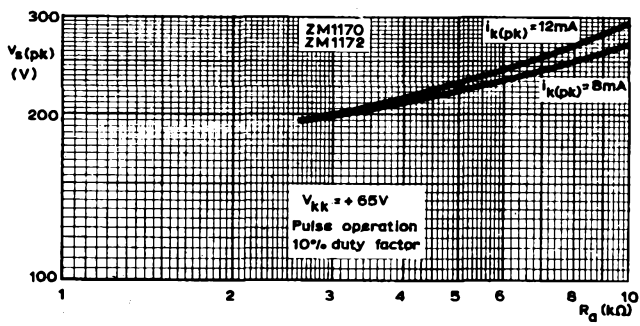
PEAK SUPPLY VOLTAGE PLOTTED AGAINST ANODE LOAD RESISTOR
