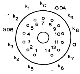
B13B Base
