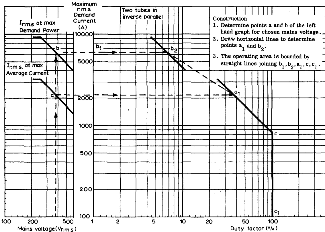
GRAPH RELATING DEMAND CURRENT WITH DUTY FACTOR AS A FUNCTION OF THE MAINS VOLTAGE. WELDING SERVICE ONLY
