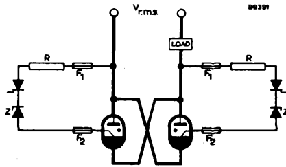
Figure 1:- Anode excitation (two thyristors)
