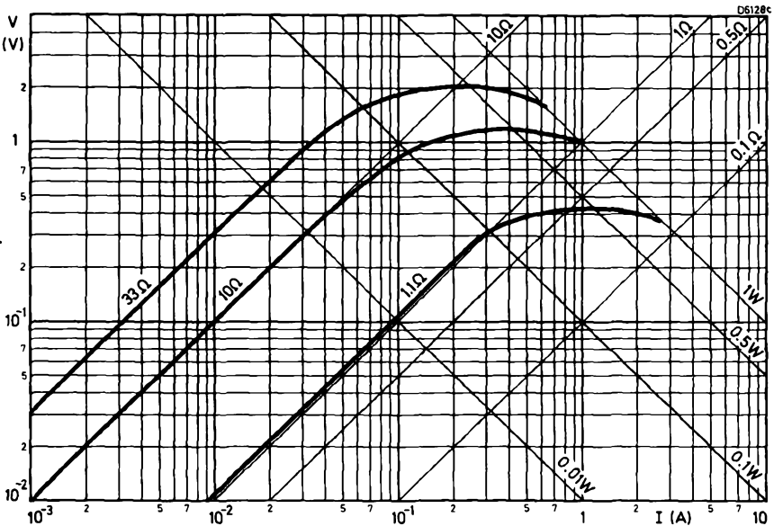
Voltage/current characteristics
