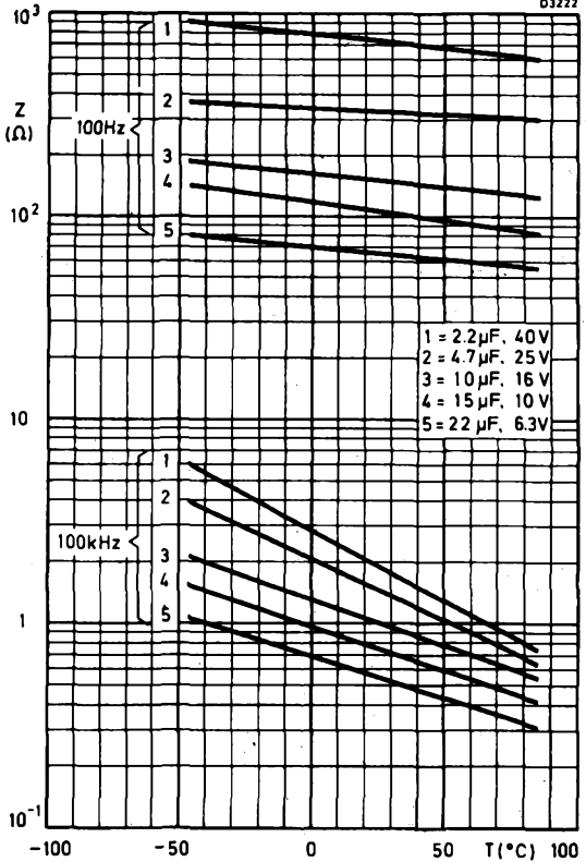
IMPEDANCE PLOTTED AGAINST TEMPERATURE WITH FREQUENCY AS PARAMETER CAN SIZE 1
