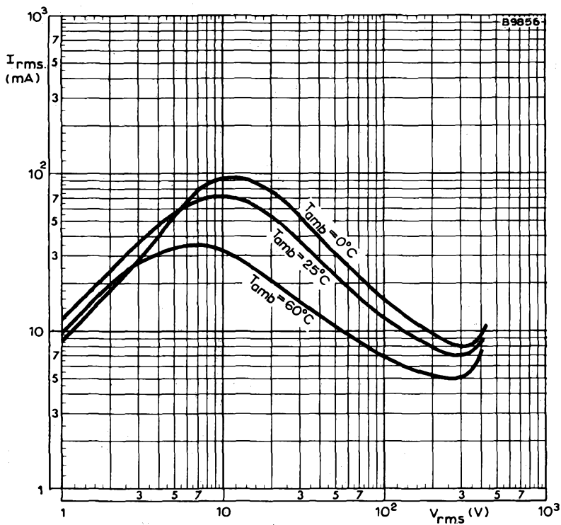
VOLTAGE/CURRENT CHARACTERISTICS
