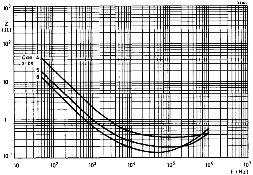
Fig.7 Typical impedance plotted against frequency, T_{amb} = 20\text{ }^{\circ}\text{C} .
