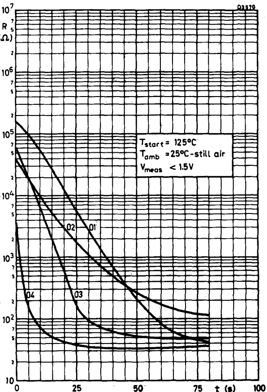
COOLING CHARACTERISTICS
