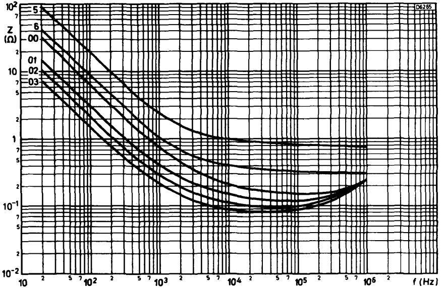
Typical impedance plotted against frequency for 16 V working capacitors, T_{amb} = 20^\circ\text{C} Can sizes 00, 01, 02, 03, 5 and 6.
