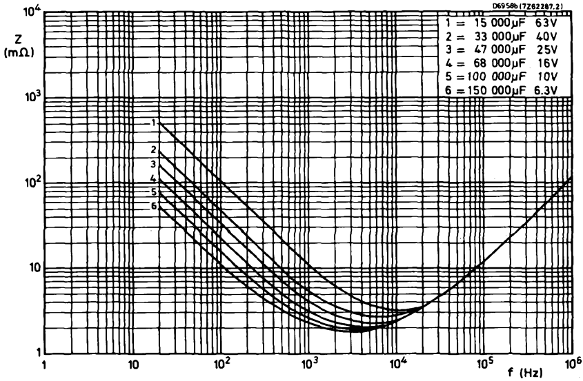
Typical impedance plotted against frequency at T_{amb} = 20^{\circ}C , can size 16
