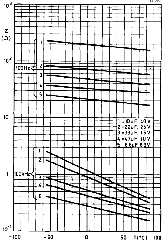
IMPEDANCE PLOTTED AGAINST TEMPERATURE WITH FREQUENCY AS PARAMETER CAN SIZE 3
