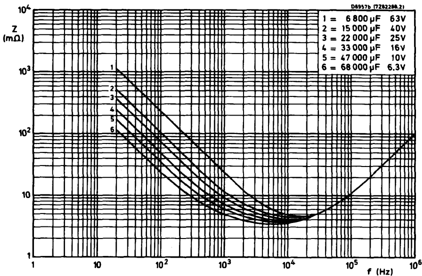
Typical impedance plotted against frequency at T_{\text{amb}} = 20^\circ\text{C} , can size 15
