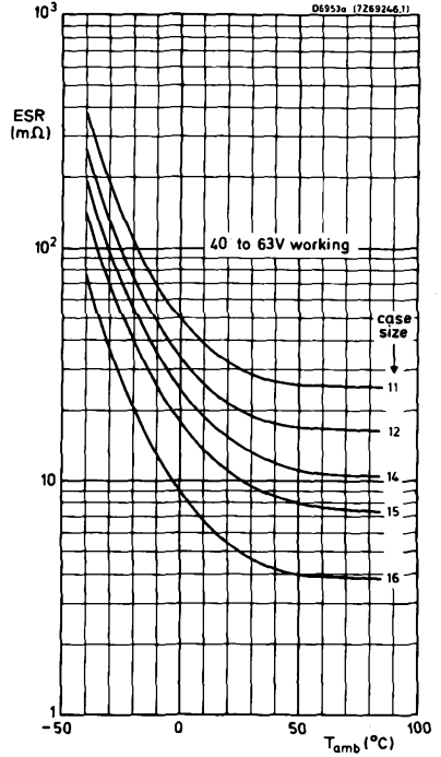
Typical ESR as a function of temperature at 100 Hz
