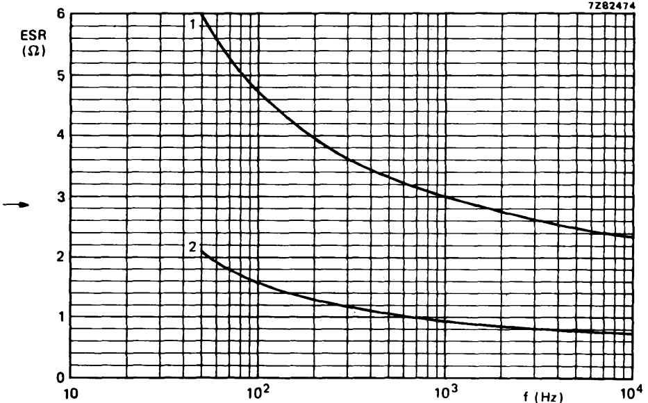
Fig. 14 Typical ESR as a function of frequency at 20 °C. Case size 02: curve 1 = 22 \mu F, 350 V; curve 2 = 47 \mu F, 160 V.
