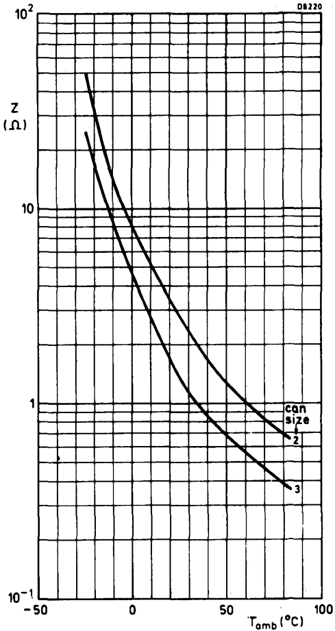
Fig.4 Impedance as a function of temperature at 100 kHz
