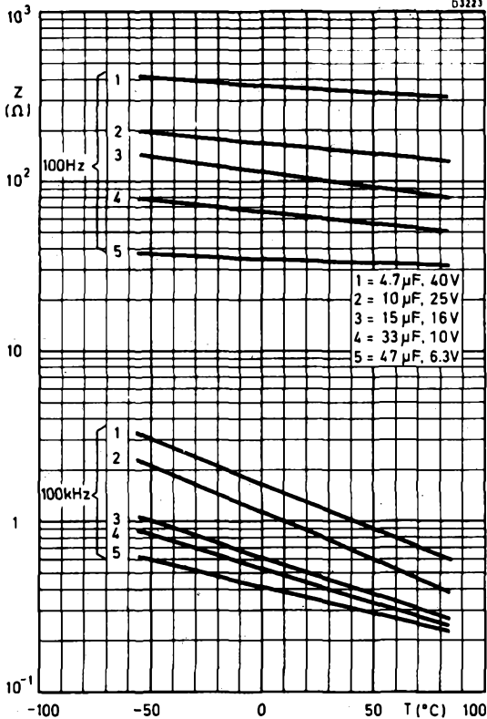
IMPEDANCE PLOTTED AGAINST TEMPERATURE WITH FREQUENCY AS PARAMETER CAN SIZE 2
