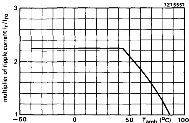
Fig. 2 Typical ripple current as a function of ambient temperature; I_{r0} = ripple current at 85 °C; 100 Hz.
