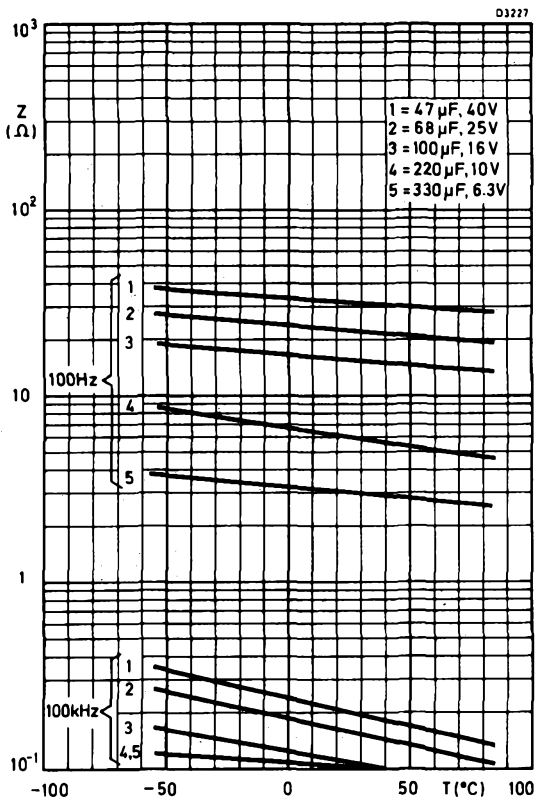
IMPEDANCE PLOTTED AGAINST TEMPERATURE WITH FREQUENCY AS PARAMETER CAN SIZE 6
