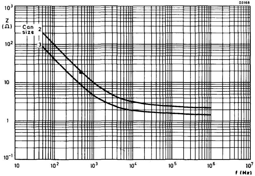
Fig.6 Typical impedance plotted against frequency, T_{amb} = 20\text{ }^{\circ}\text{C}
