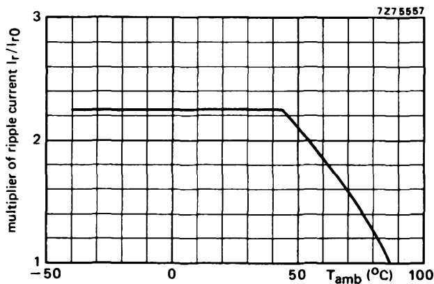
Fig. 5 Typical ripple current as a function of ambient temperature; I_{r0} = ripple current at 85\text{ }^{\circ}\text{C} , 100\text{ Hz} .
