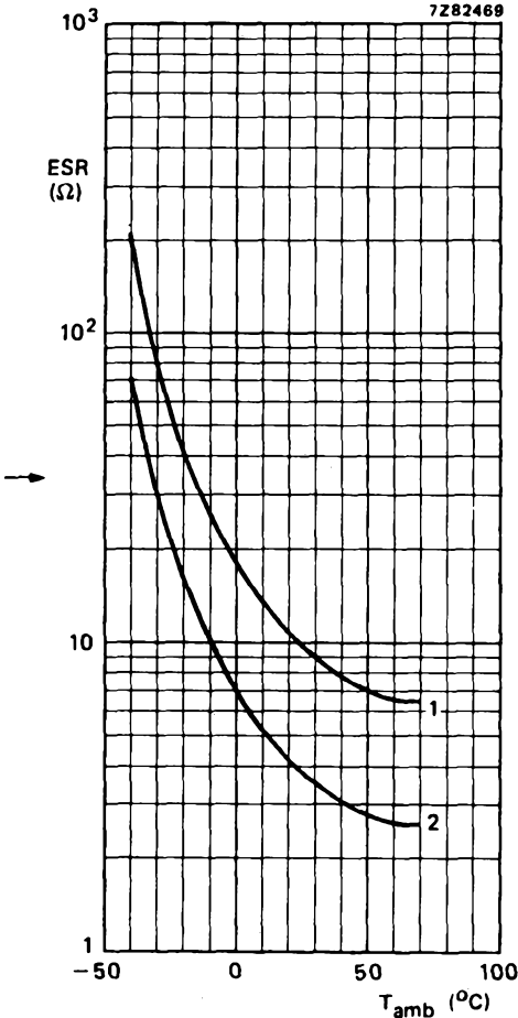
Fig. 9 Typical ESR as a function of ambient temperature at 100 Hz.
