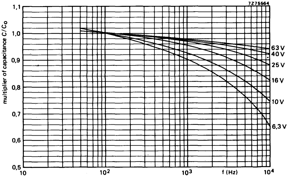
Fig. 4 Typical capacitance as a function of frequency; C_0 = capacitance at 25\text{ }^{\circ}\text{C} , 100 Hz.
