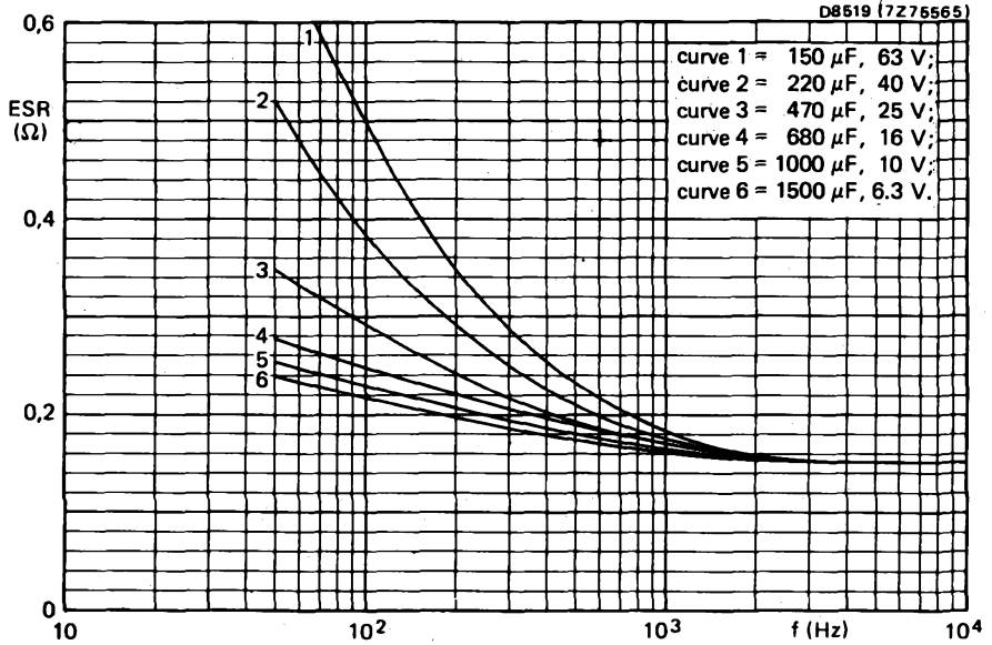
Fig.16 Typical ESR as a function of frequency at 25 °C
