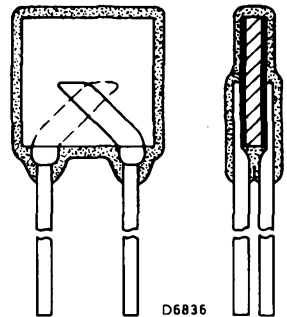
Fig. 2 Single plate capacitor
