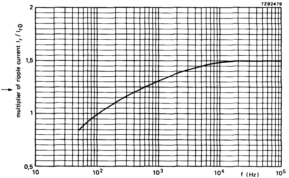
Fig. 6 Typical ripple current as a function of frequency; I_{r0} = ripple current at 70^{\circ}\text{C} , 100 Hz.
