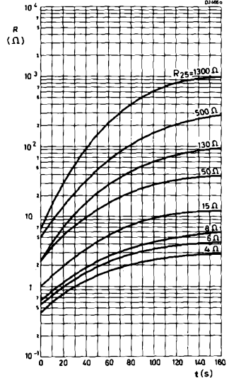
Cooling characteristics
