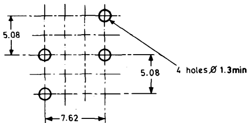
Printed wiring board piercing diagram
