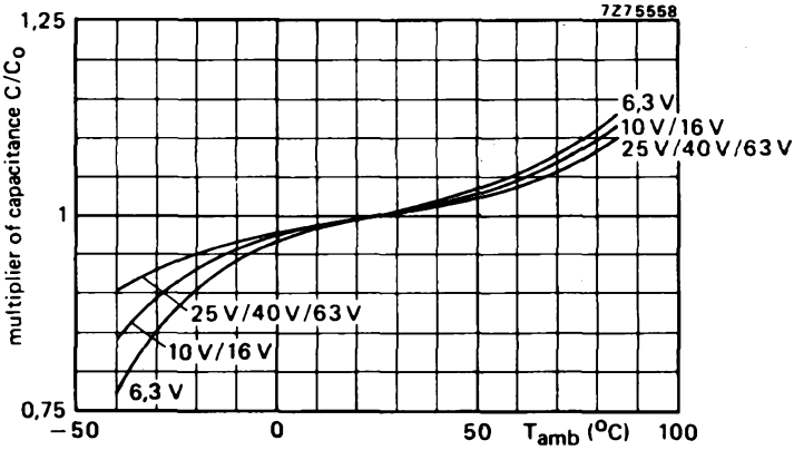
Fig. 3 Typical capacitance as a function of ambient temperature; C_0 = capacitance at 25\text{ }^{\circ}\text{C} , 100 Hz.
