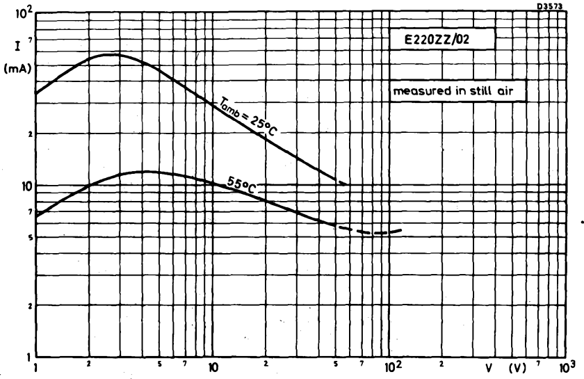
VOLTAGE/CURRENT CHARACTERISTICS
