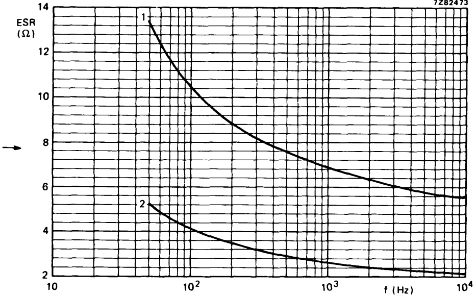
Fig. 13 Typical ESR as a function of frequency at 20 °C. Case size 01: curve 1 = 10 \mu F, 350 V/385 V; curve 2 = 22 \mu F, 250 V.
