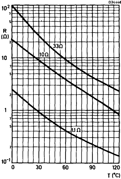
Resistance/temperature characteristics
