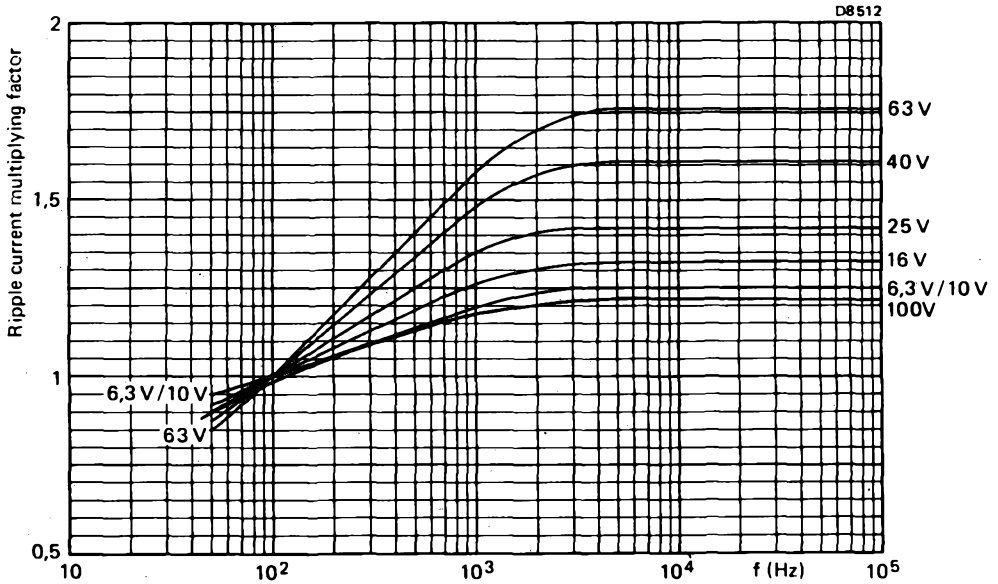
Fig.8 Typical ripple current as a function of frequency
