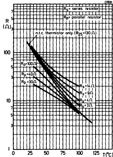
Fig. 8 Resistance as a function of temperature of a thermistor with R_{25} = 130\Omega , in series or parallel with various resistors
