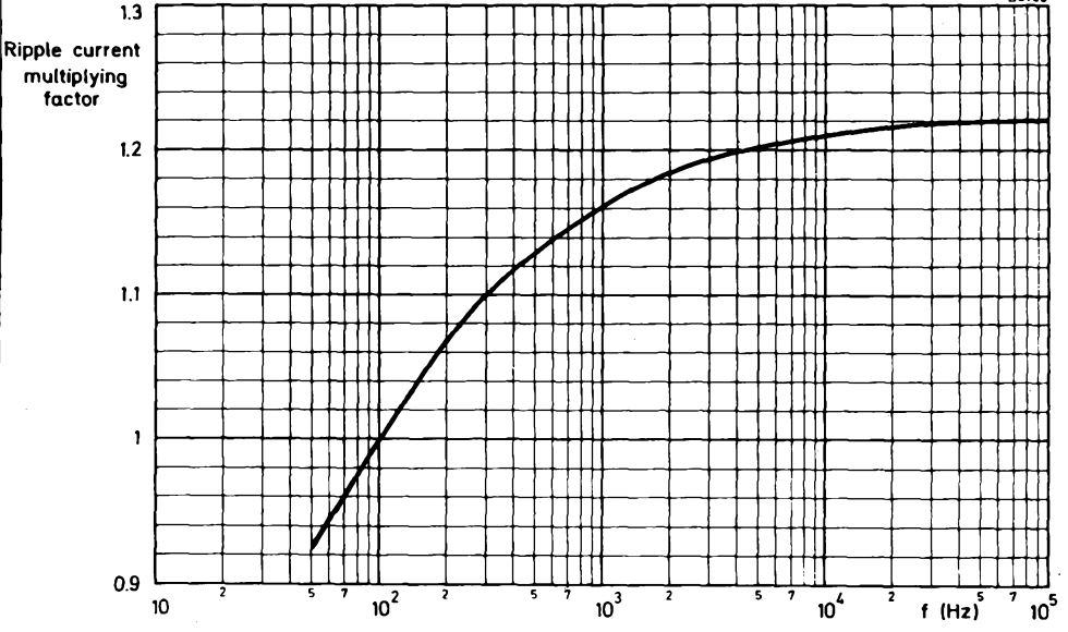
Typical ripple current multiplying factor plotted against frequency
