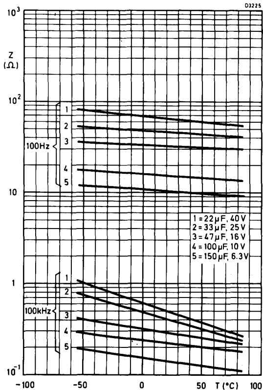
IMPEDANCE PLOTTED AGAINST TEMPERATURE WITH FREQUENCY AS PARAMETER CAN SIZE 4
