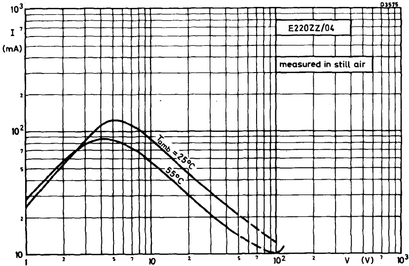
VOLTAGE/CURRENT CHARACTERISTICS
