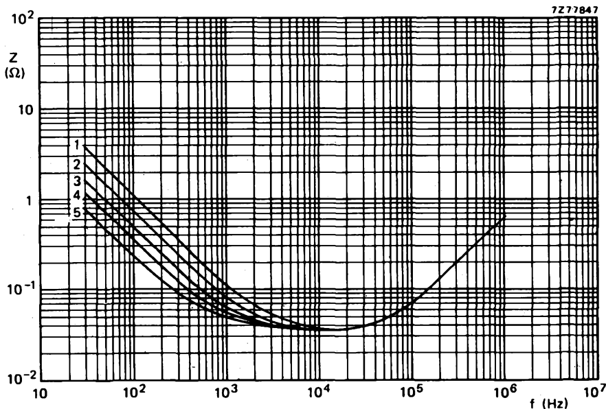
Fig. 13 Typical impedance as a function of frequency at 25 °C. Case size 04:
