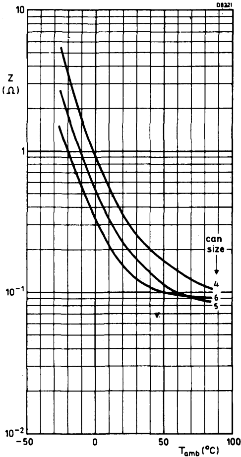
Fig.5 Impedance as a function of temperature at 100 kHz
