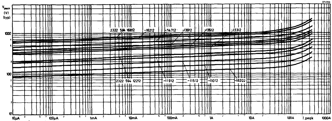
Fig. 1 Typical voltage versus current characteristic
