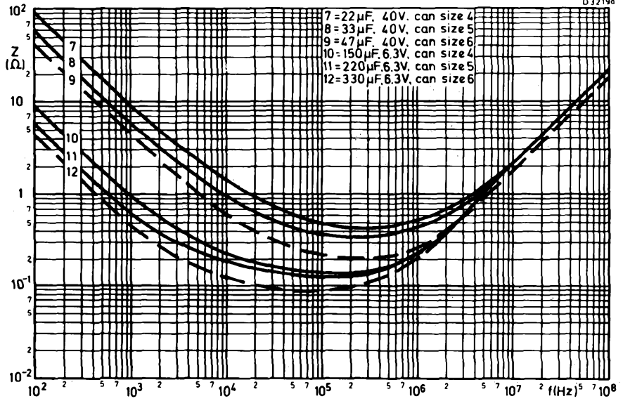
IMPEDANCE PLOTTED AGAINST FREQUENCY AT T_{amb} = 20^{\circ}\text{C} (CAN SIZES 4, 5 AND 6)
