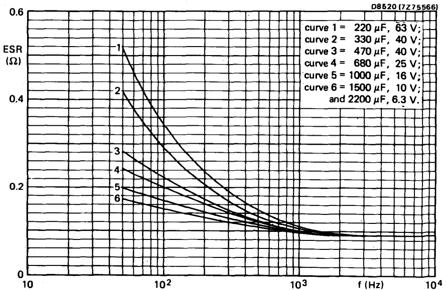
Fig.17 Typical ESR as a function of frequency at 25 °C
