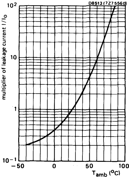
Fig.9 Typical leakage current as a function of ambient temperature; I_0 = leakage current during continuous operation at 25 ^{\circ}\text{C} and U_R .
