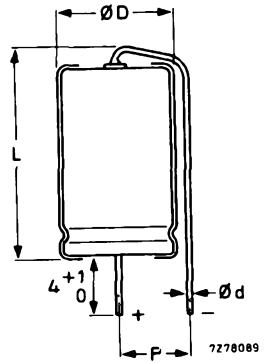
Fig. 3 Style 3; see Table 1b for dimensions d, D, L and P.
