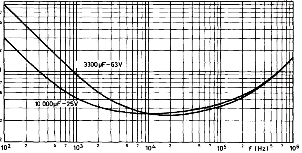
Typical impedance plotted against frequency. T_{\text{amb}} = 20^\circ\text{C}
