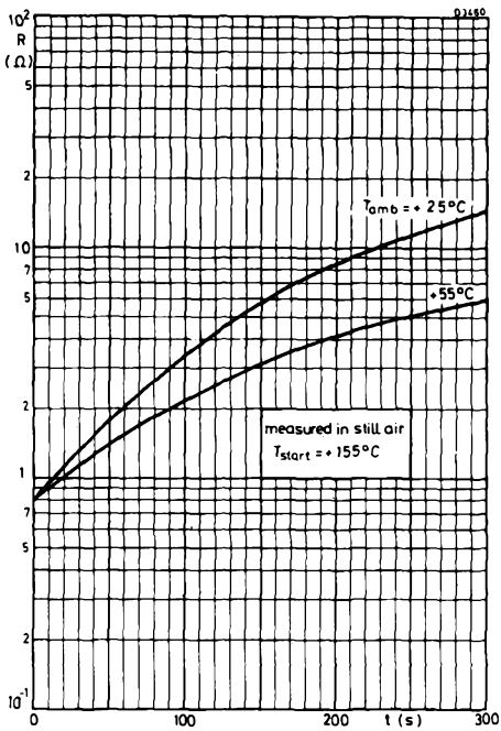
COOLING CHARACTERISTICS
