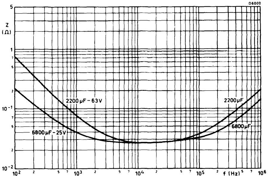
Typical impedance plotted against frequency. T_{amb} = 20^\circ C
