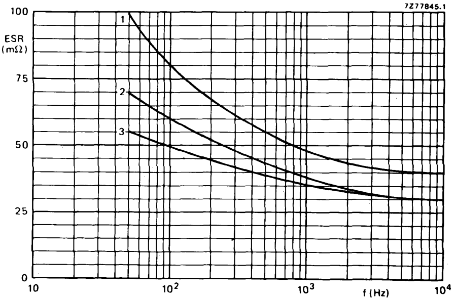
Fig. 12 Typical ESR as a function of frequency at 25 °C. Case size 05: curve 1 = 1000 μF, 63 V; curve 2 = 2200 μF, 40 V and 3300 μF, 25 V; curve 3 = 4700 μF, 16 V, 6800 μF, 10 V and 10 000 μF, 6,3 V.
