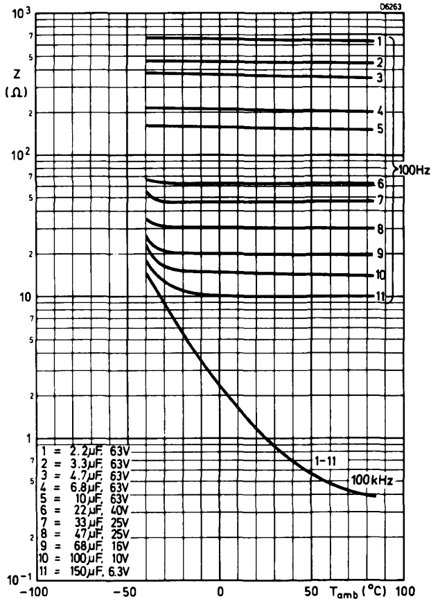
Impedance plotted against temperature with frequency as a parameter. Can size 5
