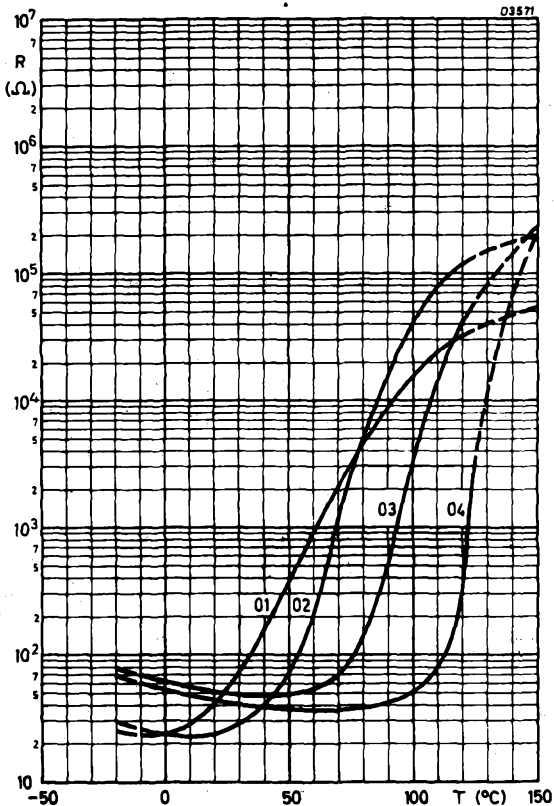
RESISTANCE/TEMPERATURE CHARACTERISTICS
