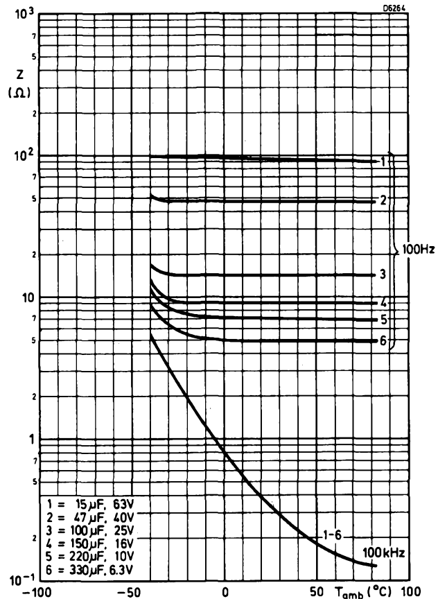
Impedance plotted against temperature with frequency as a parameter. Can size 6
