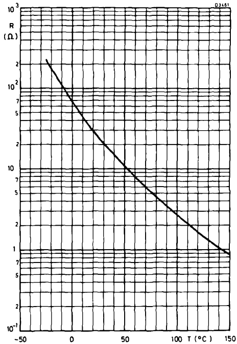
RESISTANCE/TEMPERATURE CHARACTERISTIC
