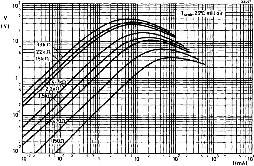
VOLTAGE/CURRENT CHARACTERISTICS
