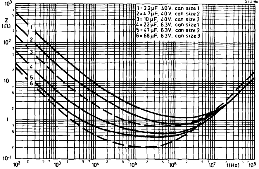
IMPEDANCE PLOTTED AGAINST FREQUENCY AT T_{amb} = 20^{\circ}\text{C} (CAN SIZES 1, 2 AND 3)
