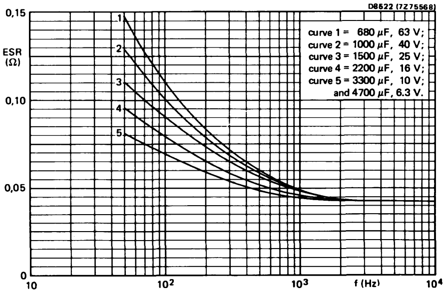
Fig.19 Typical ESR as a function of frequency at 25 °C
