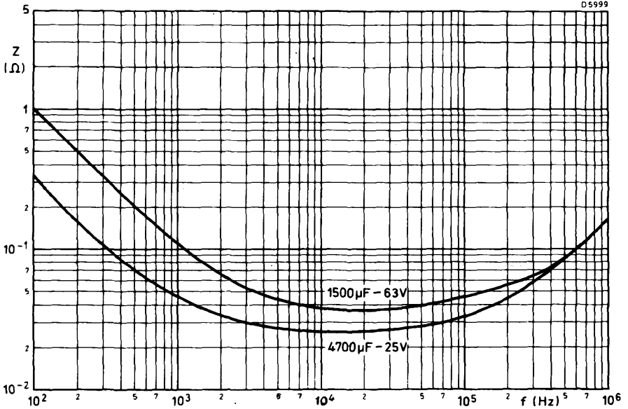
Typical impedance plotted against frequency. T_{amb} = 20^\circ C
