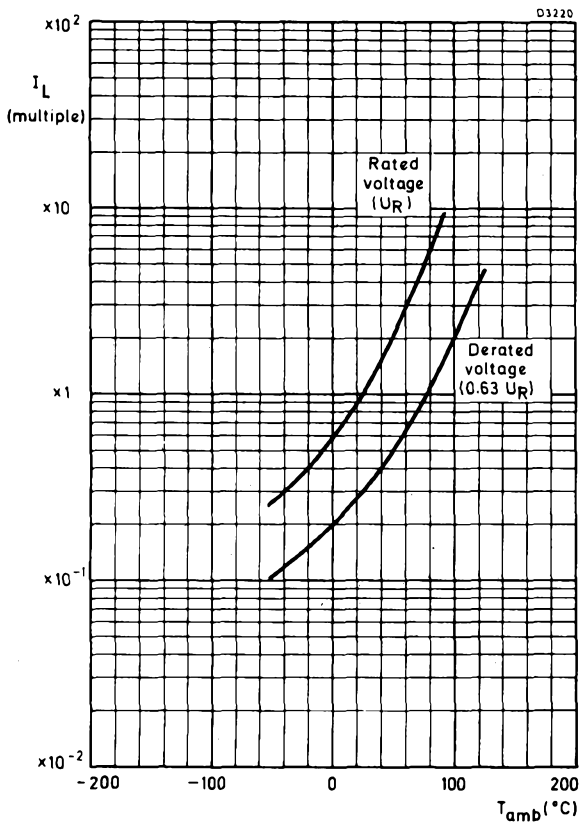
MULTIPLE OF LEAKAGE CURRENT (I_L \text{ for } T_{amb} = 20^{\circ}\text{C}) PLOTTED AGAINST AMBIENT TEMPERATURE
