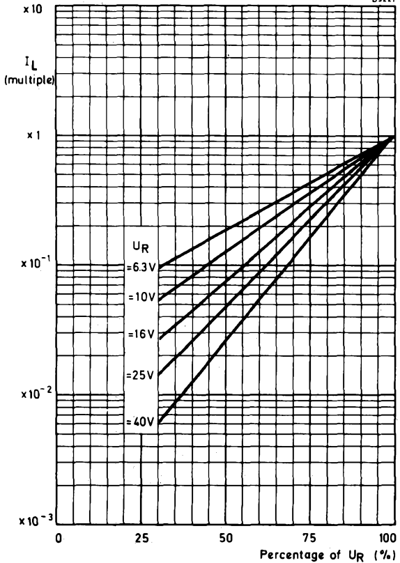
MULTIPLE OF LEAKAGE CURRENT ( I_L for T_{amb} = 20^{\circ}C ) PLOTTED AGAINST PERCENTAGE OF RATED VOLTAGE APPLIED
