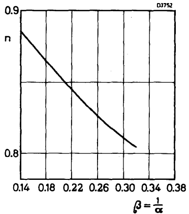
Fig. 10 Relation between the voltage caused by a d. c. current I and an a. c. current I_{\text{r.m.s.}} = I
