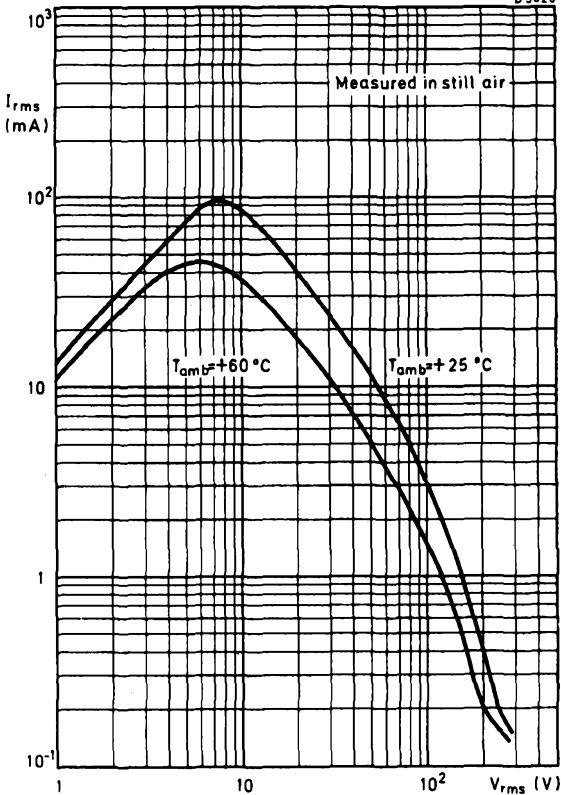
STATIC CURRENT THROUGH THE COIL/VOLTAGE CHARACTERISTICS
