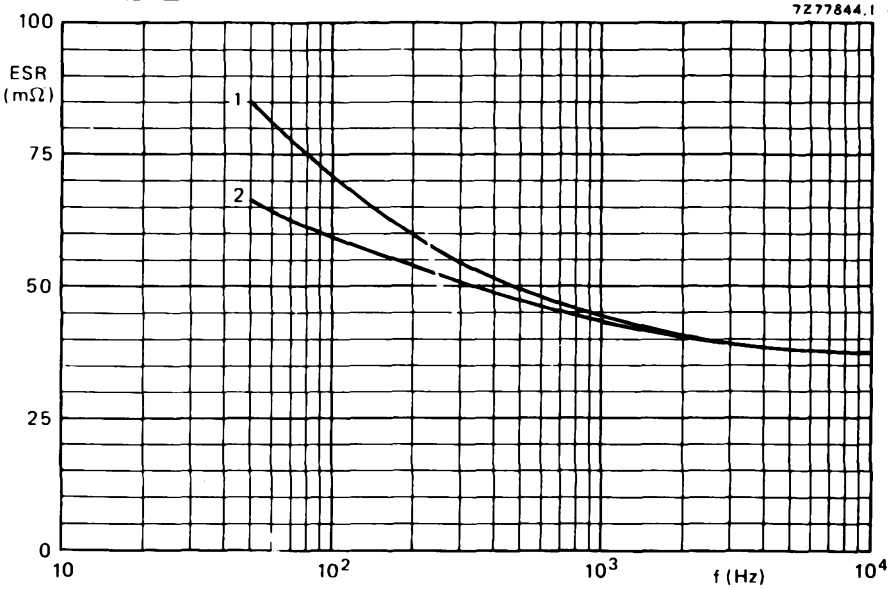
Fig. 11 Typical ESR as a function of frequency at 25 °C. Case size 04: curve 1 = 1500 μF, 40 V and 2200 μF, 25 V; curve 2 = 3300 μF, 16 V, 4700 μF, 10 V and 6800 μF, 6,3 V.
