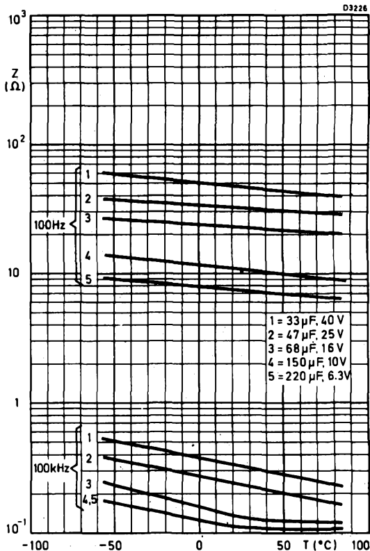
IMPEDANCE PLOTTED AGAINST TEMPERATURE WITH FREQUENCY AS PARAMETER CAN SIZE 5
