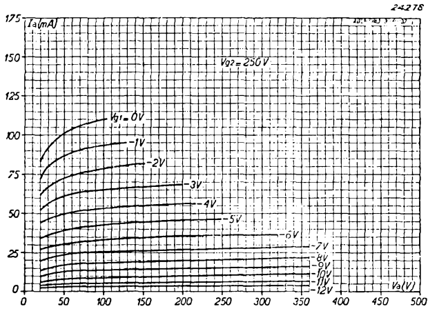
Fig. 4 Anode current as a function of the anode voltage at V_{g2} = 250V and at different values of grid bias.
