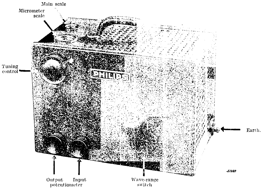
Fig. 1 Philips heterodyne wavemeter GM 3110.
