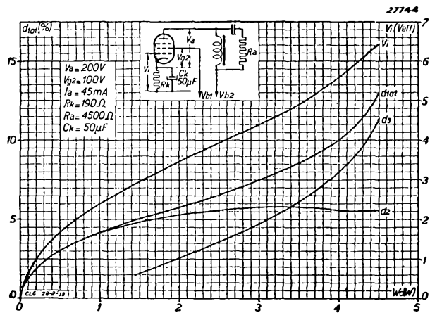
Fig. 7 Total distortion, 2nd and 3rd harmonic distortion and alternating grid voltage; CL 6 used as single output valve with automatic bias. V_a = 200 V , V_{g2} = 100 V .
