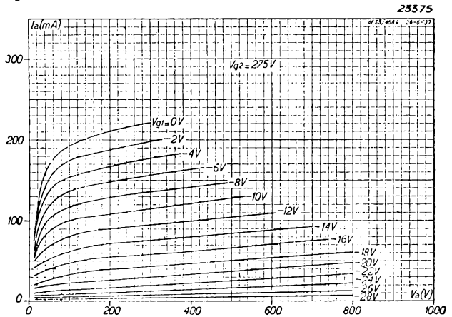
Fig. 4 Anode current of the 4689 as a function of the anode voltage for different values of grid bias. V_{g2} = 275 V.
