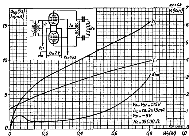
Fig. 7 Alternating grid voltage V_i , total distortion and combined anode current of the output power of two KL 4 valves in a balanced circuit operating without grid current ( V_a = V_{g2} = 135V ).
