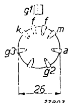
Fig. 2 Arrangement of electrodes and base connections.
