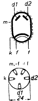
Fig. 2 Arrangement of electrodes and base connections.
