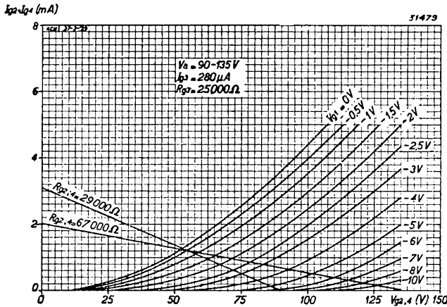
Fig. 14 Screen-grid current I_{g2} + I_{g4} as a function of the screen voltage V_{g2,4} with grid bias V_{g1} as parameter. The resistance lines for R_{g2,4} = 67,000 ohms for a battery voltage of 135 V, and for V_{g2,4} with reference to a 90 V battery are also given.
