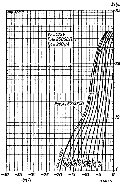
Fig. 4 Conversion conductance as a function of the grid bias, with the screen voltage as parameter. The broken line refers to the conductance when control is applied to the valve, with the screen fed from the 135 V battery through a resistor of 67,000 ohms.
