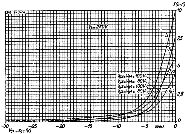
Fig. 8 Anode and screen-grid current as a function of the voltage on grids 1 and 3 when using the EH 2 as R.F. or I.F. amplifier.
