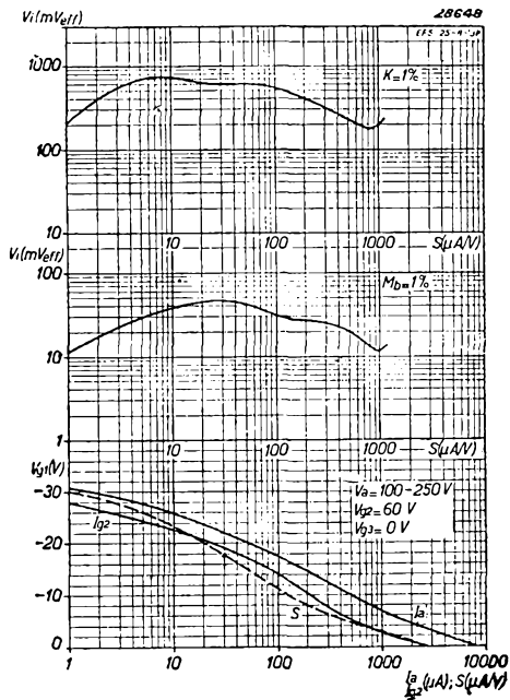
Fig. 7 At 100-250 V anode and 60 V screen: Upper diagram. Effective alternating grid voltage as a function of the mutual conductance, with 1% cross-modulation. Centre diagram. Effective alternating grid voltage as a function of the mutual conductance, with 1% modulation hum. Lower diagram. Mutual conductance S , anode current I_a and screen current I_{g2} as a function of the grid bias.
