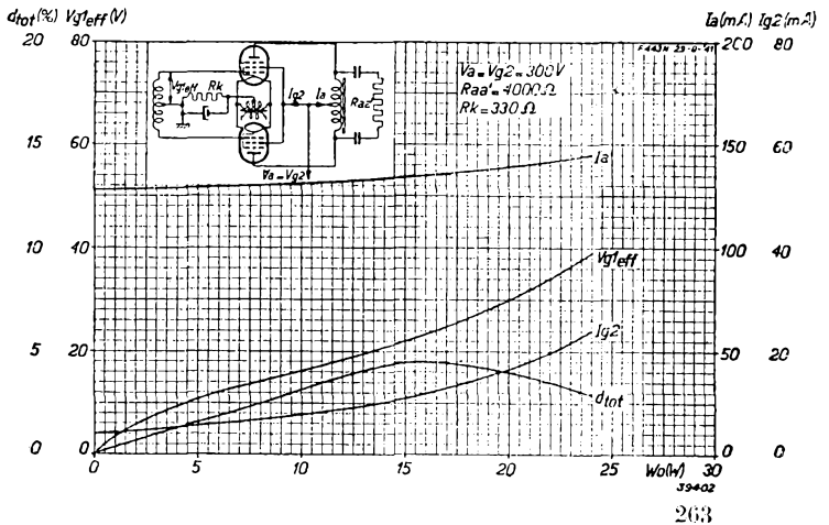
Fig. 9 Total distortion, total anode and screen-grid current and alternating grid voltage as functions of the output power. Two F 443 N valves in a balanced output stage with automatic bias. V_a = V_{g2} = 300 V .
