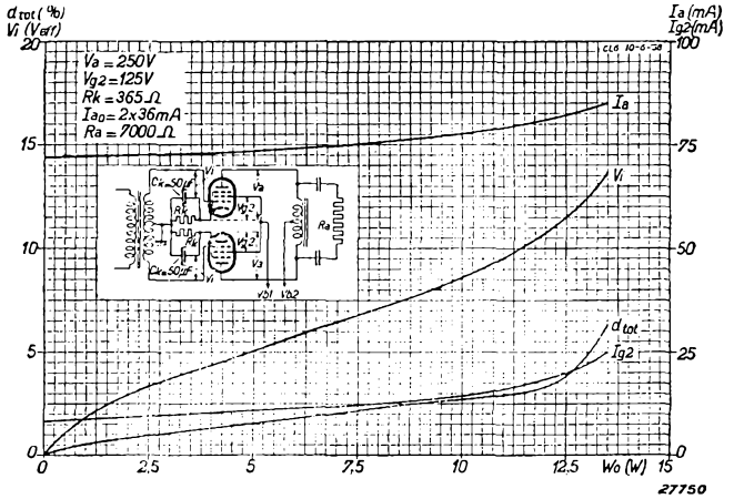
Fig. 13 Anode current I_a , screen current I_{g2} , total distortion d_{tot} and alternating grid voltage V_1 as functions of the output power for two type CL 6 valves in a balanced circuit with V_a = 250\text{ V} , and V_{g2} = 125\text{ V} .
