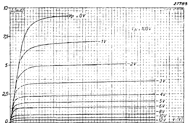
Fig. 5 Anode current as a function of the anode voltage at different values of grid bias and with a fixed screen potential of 100 V.
