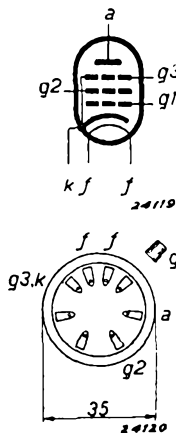
Fig. 2 Arrangement of electrodes and base connections.
