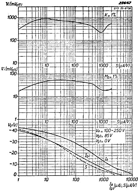
Fig. 6 At 100-250 V anode and 85 V screen; Upper diagram. Effective alternating grid voltage as a function of the mutual conductance, with 1% cross modulation. Centre diagram. Effective alternating grid voltage as a function of the mutual conductance, with 1% modulation hum. Lower diagram. Mutual conductance S , anode current I_a and screen current I_{g2} as a function of the grid bias.
