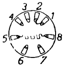
Fig. 5 Base connections of the C 3 and C 8. Contacts 1 and 2 are connected together so that A.C./D.C. receivers can be switched for high voltage mains.
