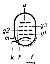
Fig. 2 Arrangement of electrodes and base connections.
