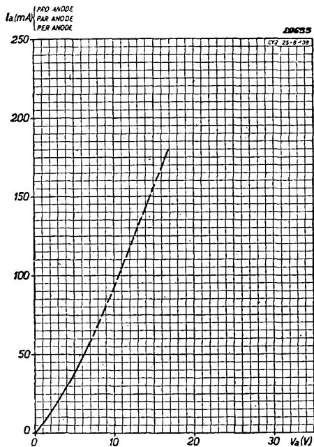
Fig. 5 Anode current as a function of the applied direct voltage, per anode.
