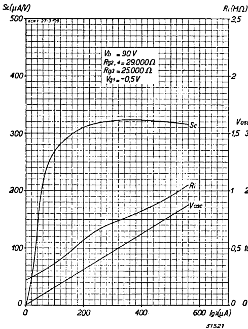
Fig. 8 Conversion conductance S_c , internal resistance R_i and effective oscillator voltage V_{osc} as functions of the oscillator-grid current I_{g3} (oscillator grid leak R_{g3} = 25,000 ohms), with V_a = 90 V and screen fed from 90 V battery through a resistor of 29,000 ohms.
