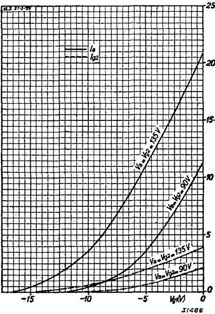
Fig. 3 Anode and screen-grid current as functions of the grid bias, with V_a = V_{g3} = 135 and 90 V.
