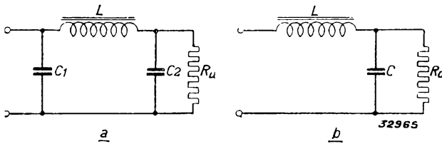
Fig. 1 a) Smoothing circuit commencing with a capacitor. b) Smoothing circuit in which the first element is a choke.
