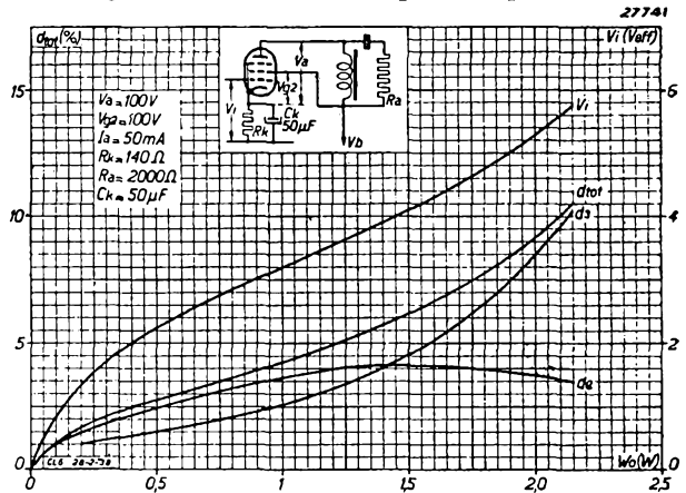
Fig. 5 Total distortion, 2nd and 3rd harmonic distortion and alternating grid voltage of the CL 6 when used as single output valve with automatic bias. V_a = V_{g2} = 100 V.
