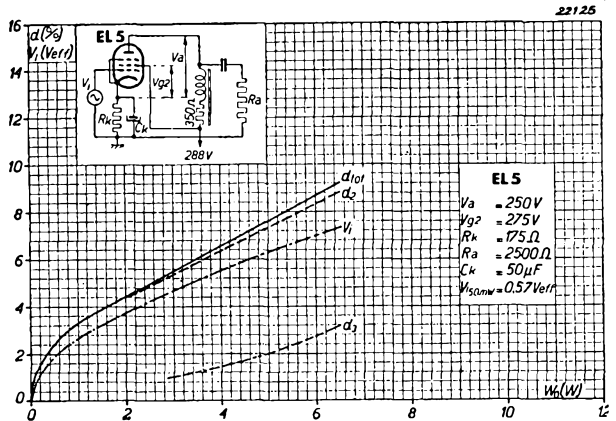
Fig. 6 Relation between alternating grid voltage, total distortion, distortion components and output power of the EL 5, with normal anode voltage, 2,500 ohms load resistor and decoupled bias resistor.
