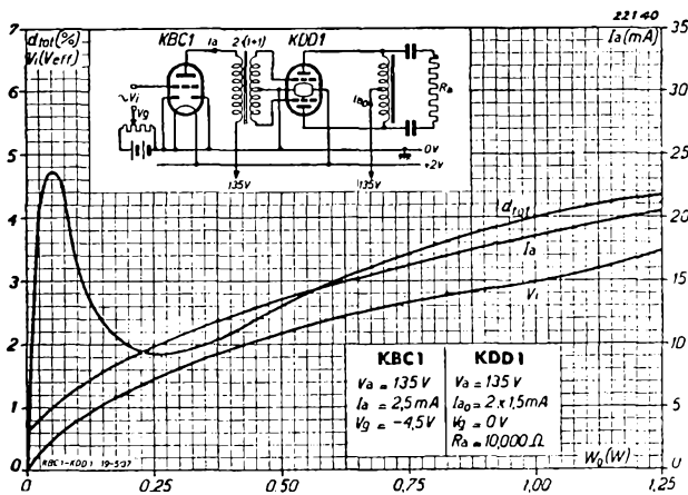
Fig. 6 Anode current, alternating grid voltage and total distortion d_{tot} as functions of the output power of the KDD 1 for an anode voltage of 135 V, using the KBC 1 as driver valve.
