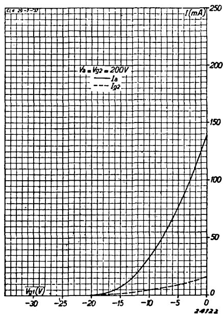
Fig. 3 Anode current as a function of the grid bias at V_a = V_{g2} = 200\text{ V} .
