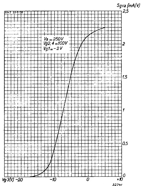
Fig. 21 Grid-current slope S_{g1a} as a function of the grid bias.
