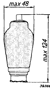
Fig. 1 Dimensions in mm.
