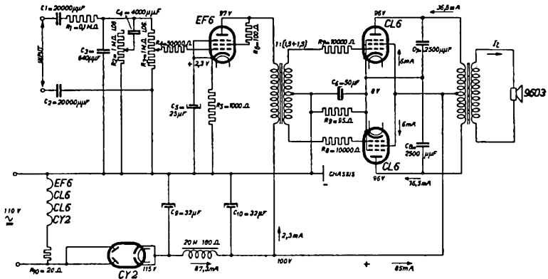
Circuit given without any guarantees with respect to patent rights.
