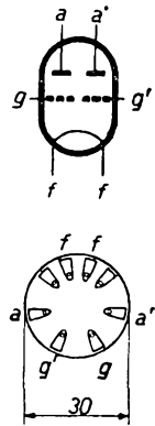
Fig. 2 Arrangement of electrodes and base connections.
