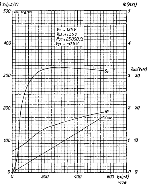
Fig. 5 Conversion conductance S_c , internal resistance R_i and effective oscillator voltage V_{osc} as functions of the oscillator-grid current I_{g3} (grid leak of oscillator, R_{g3} = 25,000 ohms), at V_a = 135 V and a fixed screen voltage of 55 V.
