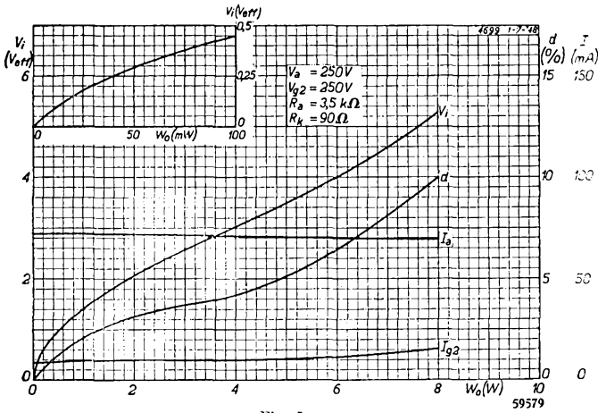
Fig. 5 Total distortion, anode and screen-grid current and alternating input voltage as functions of the output power; the 4699 used as single output valve class A with V_a = 250V and V_{g2} = 250V .
