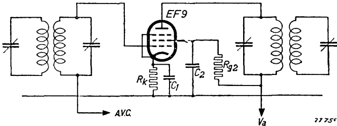
Fig. 5 Theoretical circuit diagram of an I.F. valve employing the principle of the "sliding" screen voltage.
