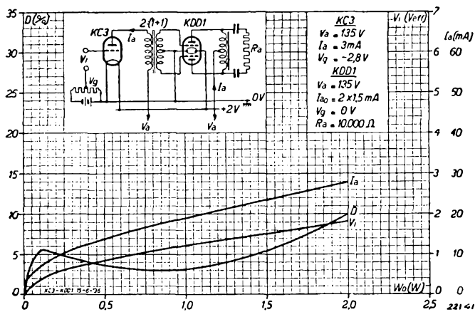
Fig. 5 Anode current, alternating grid voltage and total distortion d_{tot} as functions of the output power of the KDD 1 for an anode voltage of 135 V, using the KC 3 as driver valve.
