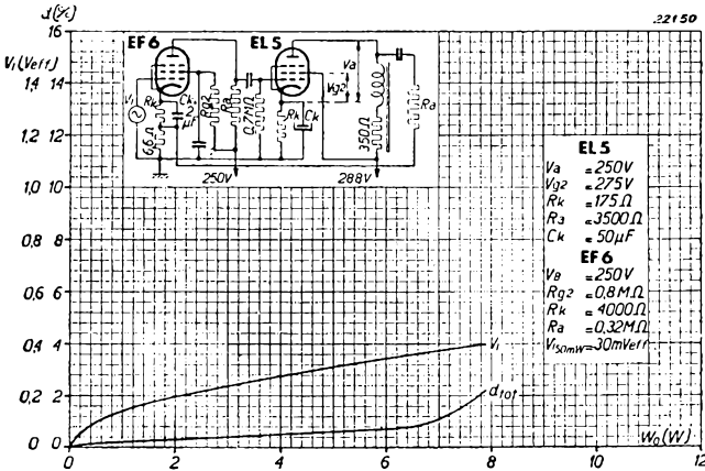
Fig. 7 Relation between alternating grid voltage V_i , total distortion d_{101} and output power; EL 5 with pre-amplifier EF 6 and negative feedback applied to the latter.
