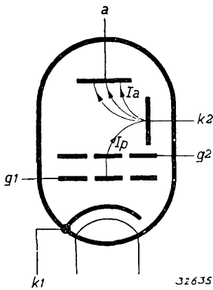
Fig. 3 Diagram of the system employed in the secondary-emission valve. Primary electrons, leaving the cathode k_1 , are deflected towards the secondary-emission cathode k_2 and the secondary electrons liberated from the latter pass to the anode. The direction followed by the electrons is shown by means of arrows and it is just the opposite to that of the stream in an ordinary receiving valve.
