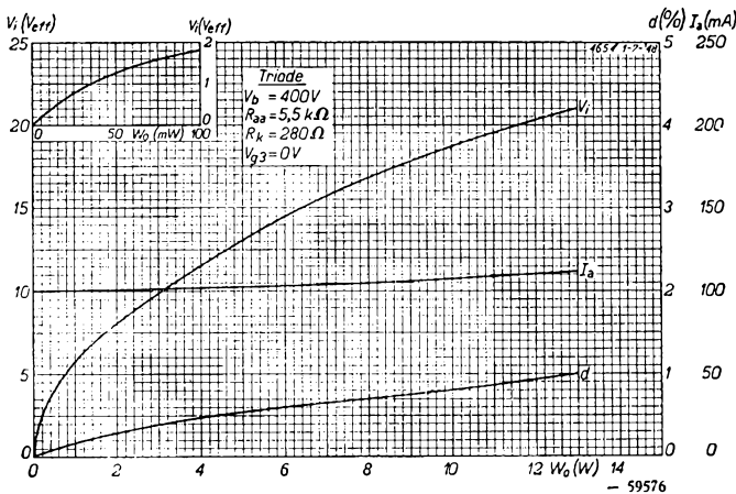
Fig. 11 Total distortion, anode current and alternating input voltage as functions of the output power; 2 valves 4654 in triode connection (screen-grid connected to anode) used in class A B output stage with V_b = 400 V
