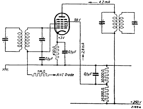
Fig. 9 Circuit diagram of the EH 2 used as an I.F. amplifier, with the same control voltage applied to grids 1 and 3.
