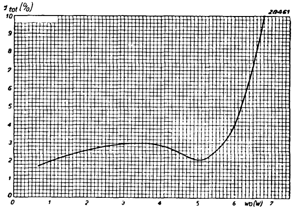
Fig. 1 Distortion in the output stage of the amplifier as a function of the output power measured at the loudspeaker.
