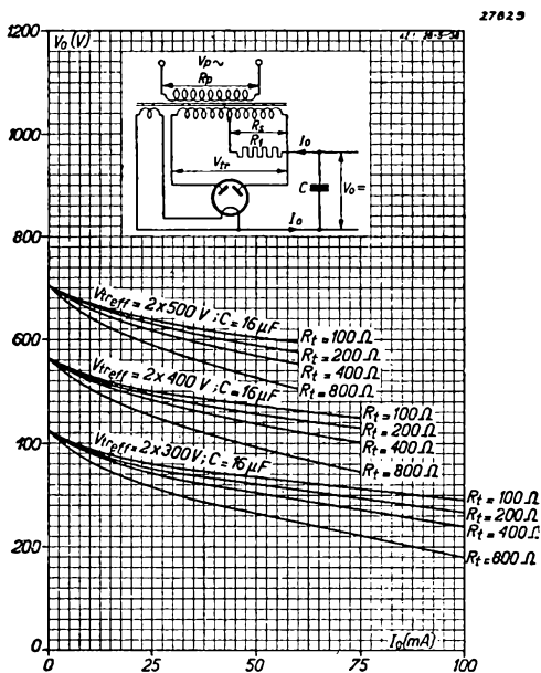
Fig. 4 Loading characteristics relating to different transformer voltages, on no load, for different values of the internal resistance of the transformer ( R_t = R_s + n^2 R_p + R_r )
