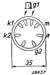
Fig. 2 Arrangement of electrodes and base connections.
