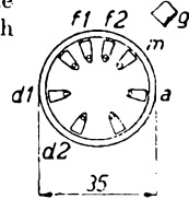
Fig. 2 Arrangement of electrodes and base connections
