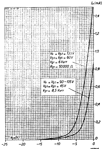
Fig. 3 Anode current as a function of the grid bias, at V_{g3,5} = 45\text{ V} and 60\text{ V} .
