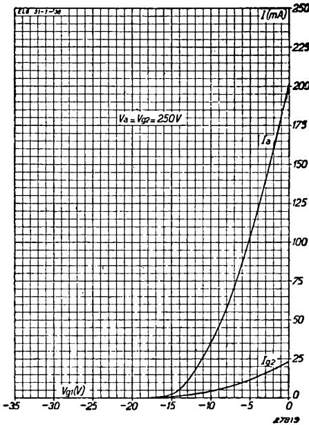
Fig. 3 Anode and screen current as a function of the grid bias, at V_a = V_{g_s} = 250 V.
