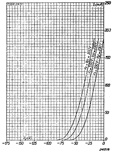
Fig. 3 Anode current as a function of the grid bias, with V_a = 550 \text{ V} , V_{g2} = 250 \text{ V} ; V_a = 550 \text{ V} , V_{g2} = 200 \text{ V} and V_a = V_{g2} = 300 \text{ V} .
