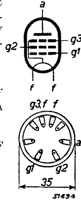
Fig. 2 Arrangement of electrodes and base connections.
