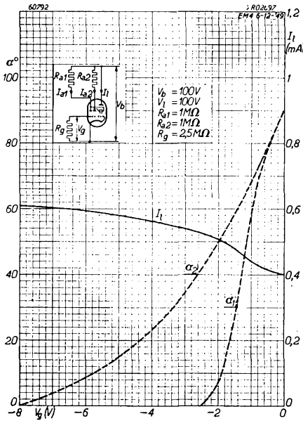
Fig. 8 Shadow angles \alpha_1 and \alpha_2 measured at the edge of the screen, and screen current I_f as functions of the grid potential
