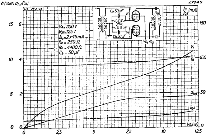
Fig. 12 Anode current I_a , screen-grid current I_{g2} , total distortion d_{tot} and alternating grid voltage V_1 , as functions of the output power W_o for two CL 6 valves in a balanced circuit with V_a = 200\text{ V} , and V_{g2} = 125\text{ V} .
