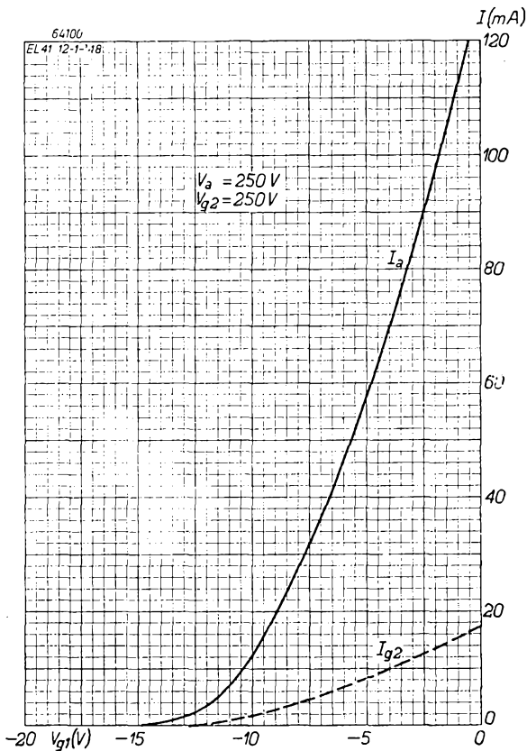
Fig. 3 Anode current I_a and screen grid current I_{g2} as functions of the grid bias V_{g1} at anode voltage V_a and screen grid voltage V_{g2} = 250 V .
