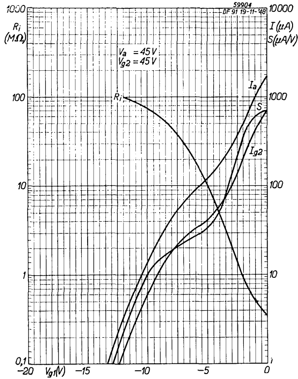
Fig. 3 Anode current ( I_a ), screen grid current ( I_{g2} ), mutual conductance ( S ) and internal resistance ( R_i ) of the DF 91 as functions of the grid bias ( V_{g1} ). Fig. 3 for V_a = V_{g2} = 45 \text{ V} ; Fig. 4 for V_a = V_{g2} = 67.5 \text{ V} .
