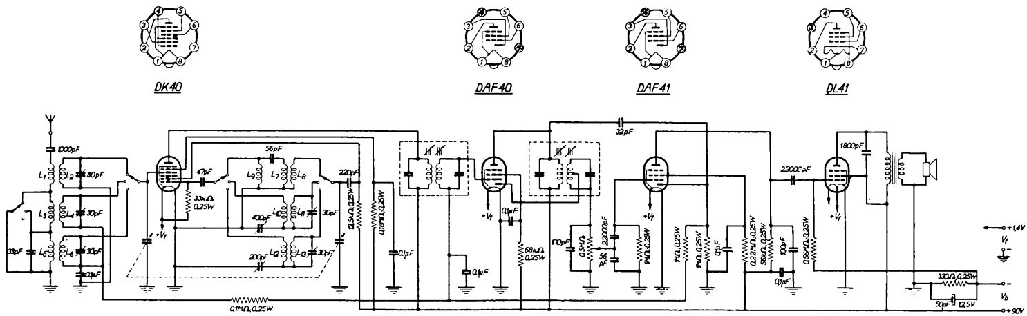
Fig. 1 Circuit of battery receiver with 4 Rimlock valves.
