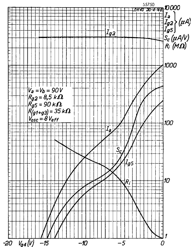
Fig. 6 Anode current ( I_a ), screen grid current ( I_{g5} ), oscillator anode current ( I_{g2} ), conversion conductance ( S_c ) and internal resistance ( R_i ) of the DK 40 as functions of the grid bias ( V_{g4} ). Measurements taken on an oscillating valve, in the circuit shown in Fig. 2.
