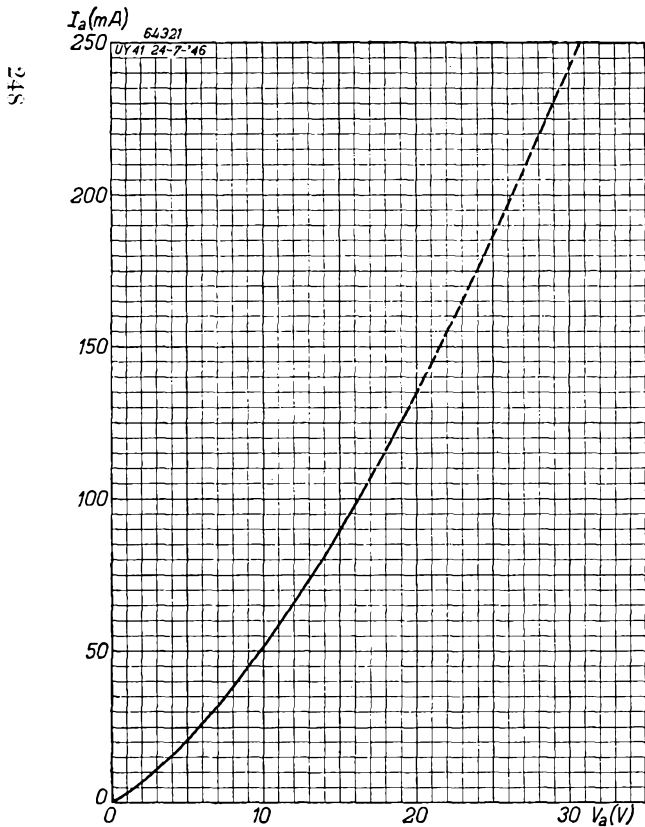
Fig. 4 Anode current ( I_a ) of the UY 41 as a function of the applied direct voltage ( V_a ).
