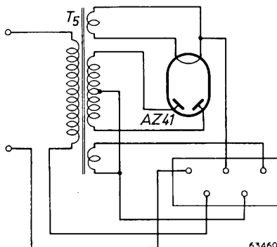
Fig. 4. Circuit of the A.C. power unit.
