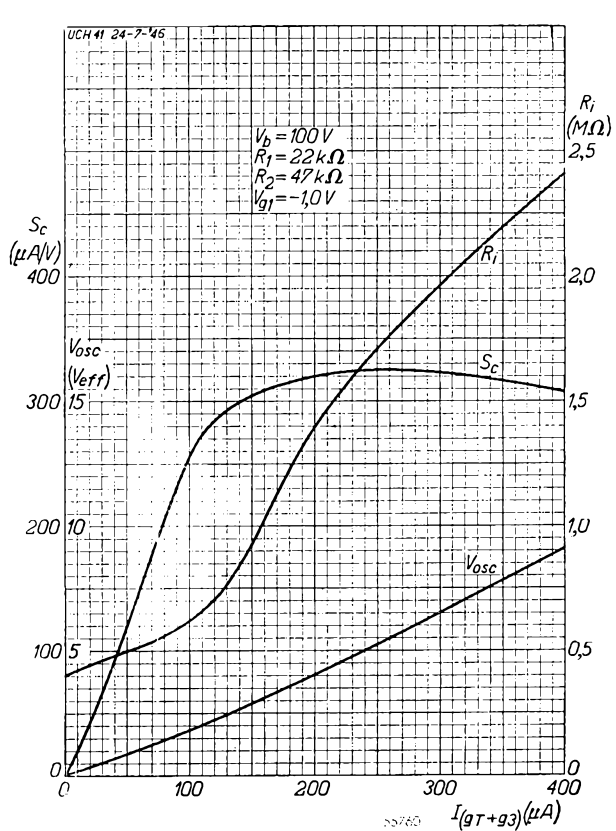
Fig. 12 Conversion conductance ( S_c ), oscillator voltage ( V_{osc} ) and internal resistance ( R_i ) of the UCH 41, as functions of the oscillator grid current ( I_{gT+g3} ). Relative to the circuit depicted in Fig. 3. Fig. 12 : V_b = 100\text{ V} ; Fig. 13 : V_b = 170\text{ V} .
