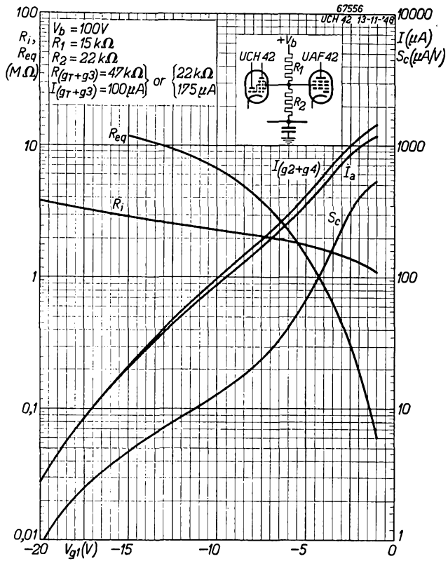
Fig. 23 As Figs. 10 and 11, but with the screen grid voltage of the UCH 42 together with that of the UAF 42 fed by means of a common potentiometer. Measured in the circuit shown in Fig. 5. Fig. 23 : supply voltage V_b = 100 V ; Fig. 24 : V_b = 170 V.
