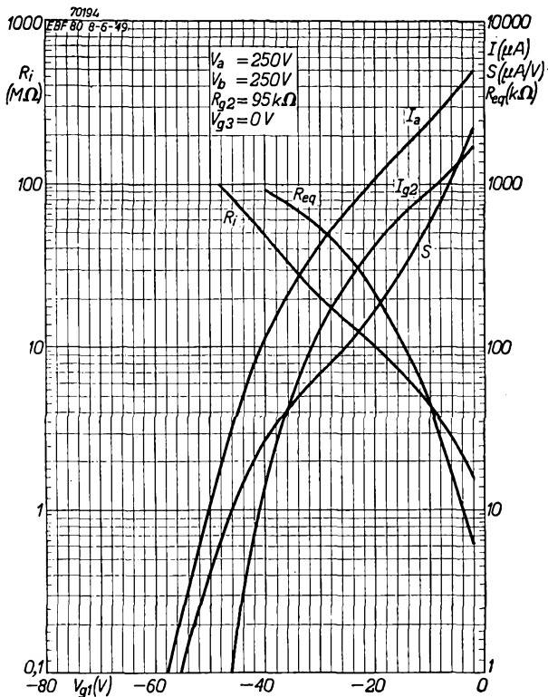
Fig. 6 Anode current ( I_a ), screen grid current ( I_{g2} ), mutual conductance ( S ), internal resistance ( R_i ) and equivalent noise resistance ( R_{eq} ) as functions of the grid bias ( V_{g1} ), with R_{g2} = 95 k\Omega in the screen grid circuit.
