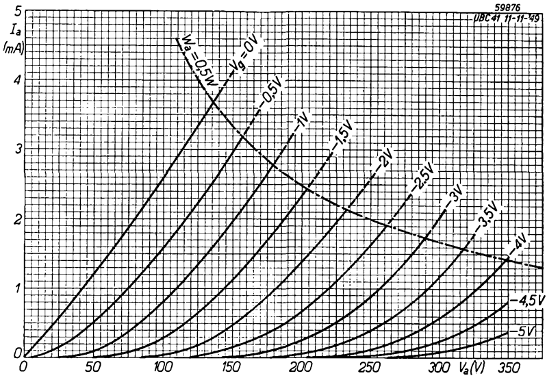
Fig. 5 I_a/V_a characteristics of the UBC 41. The dot-dash line indicates the maximum permissible anode dissipation ( I V_a = 0.5W ).
