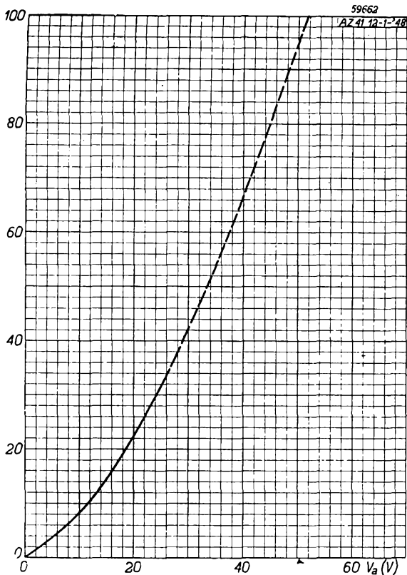
Fig. 3. Anode current ( I_a ) per anode as a function of the anode voltage ( V_a ). As the maximum permissible current is 35 mA per anode, the curve above this point is shown by a dotted line.
