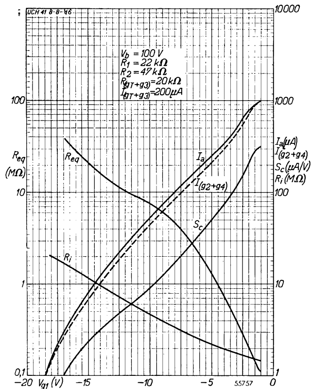
Fig. 10 Anode current ( I_a ), screen grid current ( I_{g_2+g_4} ), conversion conductance ( S_c ), internal resistance ( R_i ) and equivalent noise resistance ( R_{eq} ) of the UCH 41, as functions of the grid bias ( V_{g_1} ). Measurements taken from oscillating valve in circuit shown in Fig. 3. Fig. 10 : V_b = 100 \text{ V} ; Fig. 11 : V_b = 170 \text{ V} .
