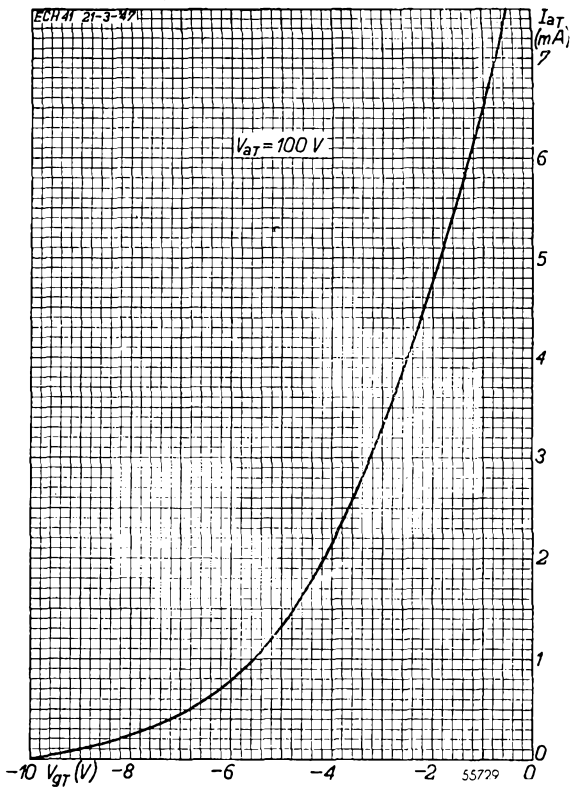
Fig. 14 Anode current I_{aT} of the triode section, as a function of the triode grid voltage V_{gT} , at an anode voltage V_{aT} = 100 \text{ V} (static characteristic).
