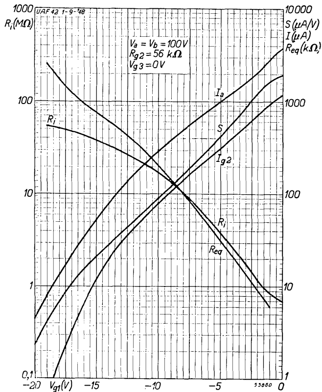
Fig. 10 Anode current ( I_a ), screen grid current ( I_{g2} ), mutual conductance ( S ), internal resistance ( R_i ) and equivalent noise resistance ( R_{eq} ) of the pentode section of the UAF 42, as functions of the grid bias ( V_{g1} ); screen grid resistor R_{g2} = 56 k\Omega , anode and supply voltage = 100 V (Fig. 10) and 170 V (Fig. 11).
