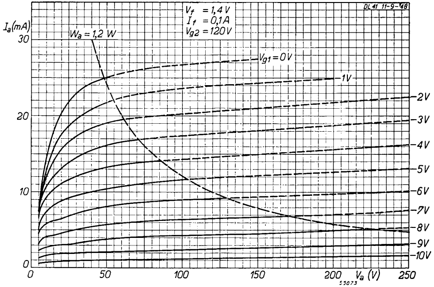
Fig. 11 As Fig. 9, but for a screen grid voltage of 120 V. Filament connections 1 and 7+8 ( V_f=1.4 V , I_f=100 mA ).
