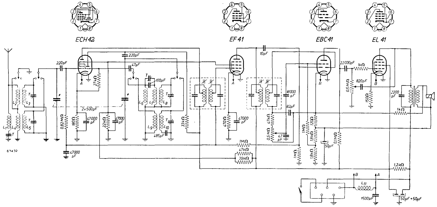
Fig. 1. Receiving circuit of a 4-valve receiver for A.C. mains and battery.
