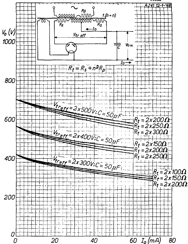
Fig. 4. Regulation curves of the AZ 41 (D.C. output voltage V_o as a function of the direct output current I_o ).
