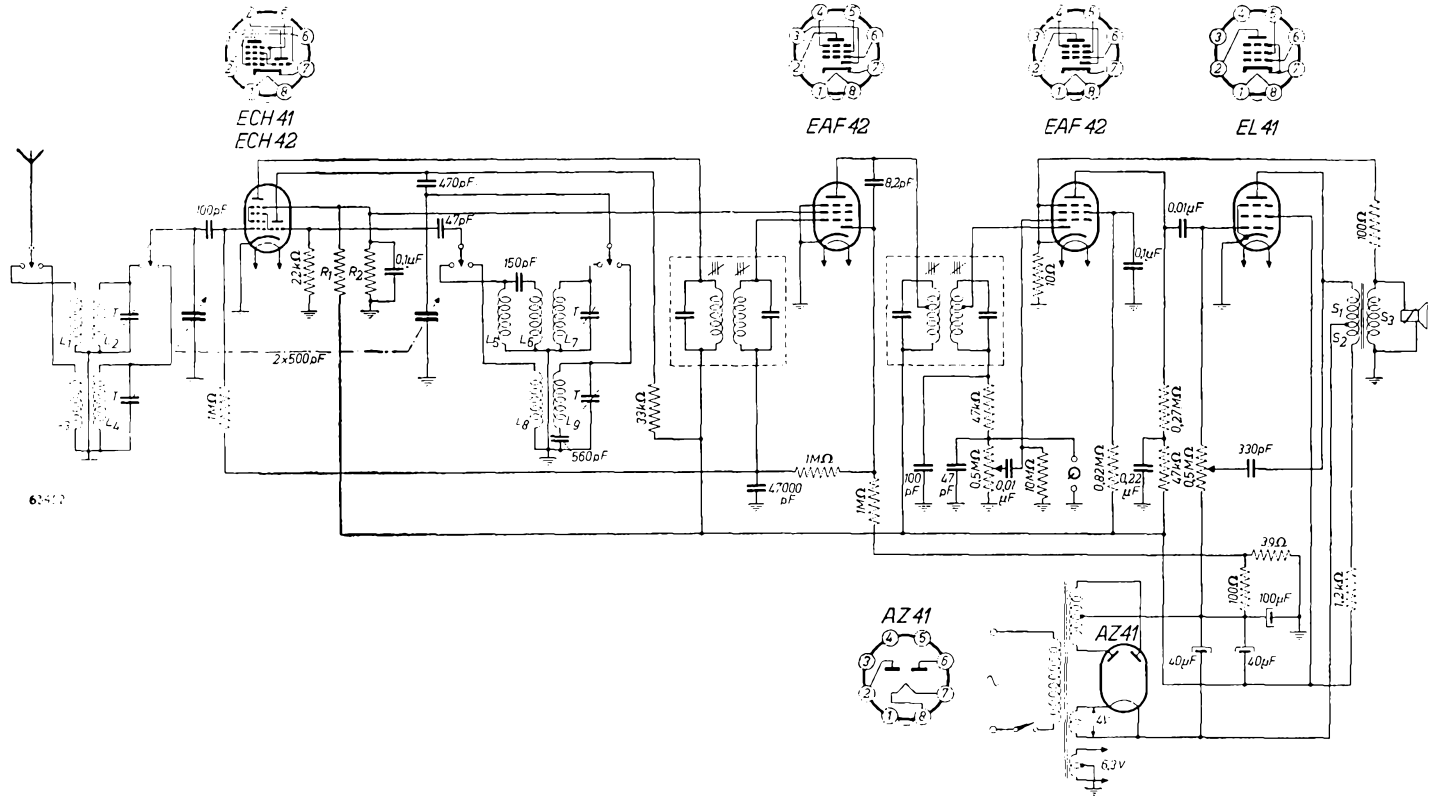
Fig. 1. Circuit of a 5-valve A.C. receiver. With ECH 41: R_1=18\text{ k}\Omega , R_2=27\text{ k}\Omega ; with ECH 42: R_1=22\text{ k}\Omega , R_2=27\text{ k}\Omega .
