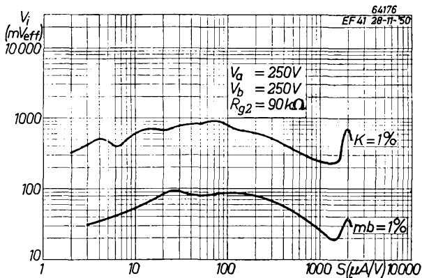
Fig. 8. The effective value V_i of an interfering signal on the control grid, producing 1% cross-modulation; also the effective value V_i of a hum signal on the control grid, producing 1% hum modulation, both as a function of the slope S .
