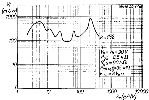
Fig. 11 Effective voltage ( V_i ) of an interfering signal on the control grid, producing 1% cross modulation, as a function of the conversion conductance ( S_c ). Upper Fig.: battery voltage 67.5 V; lower Fig.: battery voltage 90 V.
