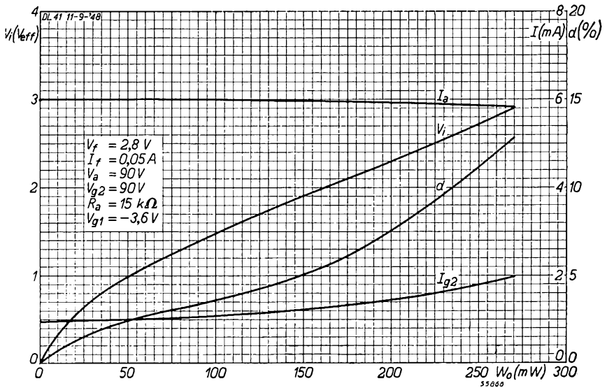
Fig. 15 Anode current ( I_a ), screen grid current ( I_{g2} ), distortion ( d ) and alternating grid voltage ( V_{ti} ) as functions of the output power ( W_o ). 90 V battery. Filament connections 7 and 8 ( V_f = 2.8 V , I_f = 50 mA ).
