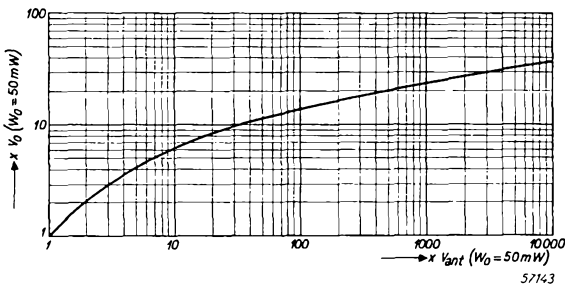
Fig. 2 A.G.C. characteristic relating to the circuit shown in Fig. 1, with an ECH 41 frequency changer.
