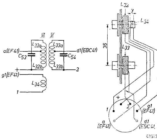
Fig. 7. Circuit and general arrangement of the third I.F. transformer. L_{32} and L_{33} are standard I.F. coils for an intermediate frequency of 452 kc/s, with 0.7 tapping. The coupling coil L_{34} contains 8 turns of wire of 0.3 mm diameter, wound in a single layer. The diameter of the can is 30 mm, the height 93 mm. The total KQ of the transformers is approximately 0.9.
