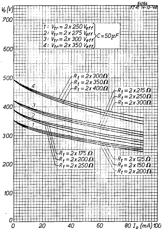
Fig. 4 Load characteristic (D.C. output voltage V_o as a function of the D.C. output current I_o ) of the EZ 40, for various values of the transformer voltage V_{tr} and different values of the D.C. resistance R_t in each anode
