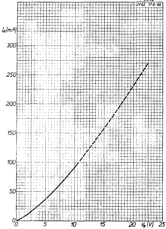
Fig. 3 Anode current ( I_a ) of the UY 42 as a function of the applied direct voltage ( V_a ).
