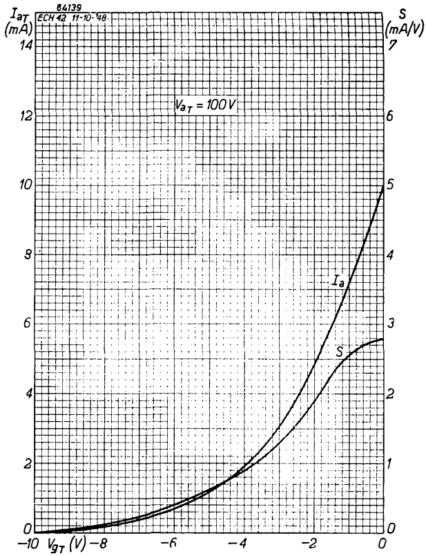
Fig. 14 Anode current ( I_a ) and slope ( S ) of the triode system as functions of the grid bias ( V_{gT} ). Measurements taken from non-oscillating valve at an anode voltage ( V_{aT} ) of 100 V.
