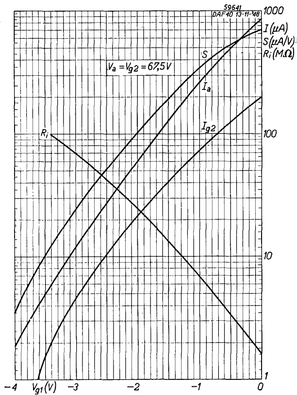
Fig. 5 Anode current ( I_a ), screen grid current ( I_{g2} ), mutual conductance ( S ) and internal resistance ( R_i ) as functions of the grid bias ( V_{g1} ) for an anode and screen grid voltage of 67.5 V (Fig. 5) and for a supply voltage of 90 V (Fig. 6).
