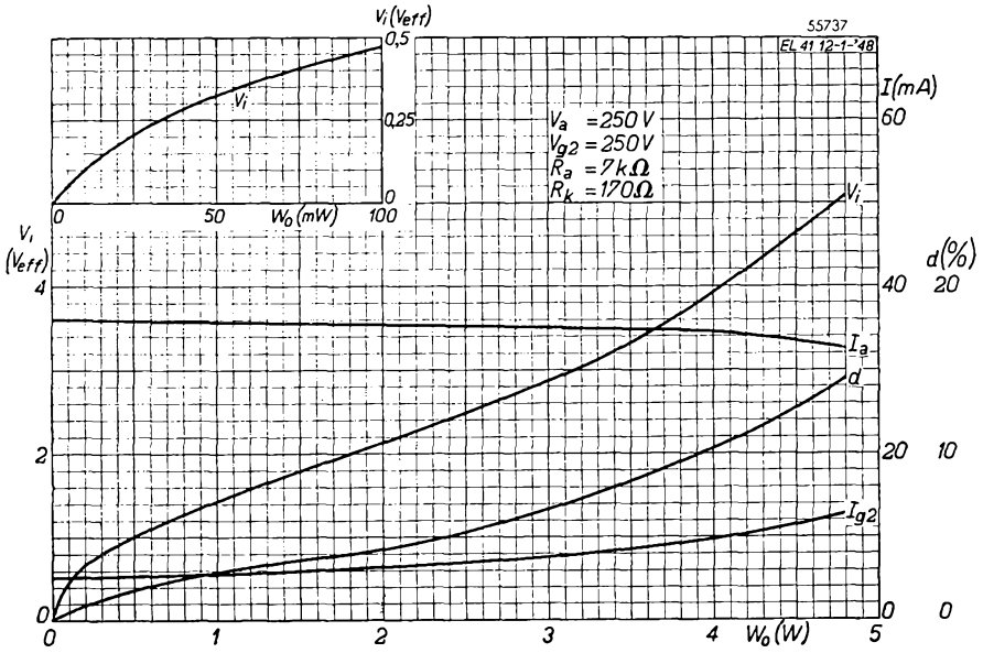
Fig. 7 Anode current I_a , screen grid current I_{g2} , distortion d and required input voltage V_i as functions of the output W_o . Upper-left inset : A.C. input voltage V_i as a function of the power output W_o for low values of W_o .
