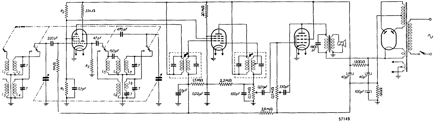
Fig. 1. A 4-valve superheterodyne A.C. receiver. The values of the resistors to be used with the ECH 42 and ECH 41 are as follows:
