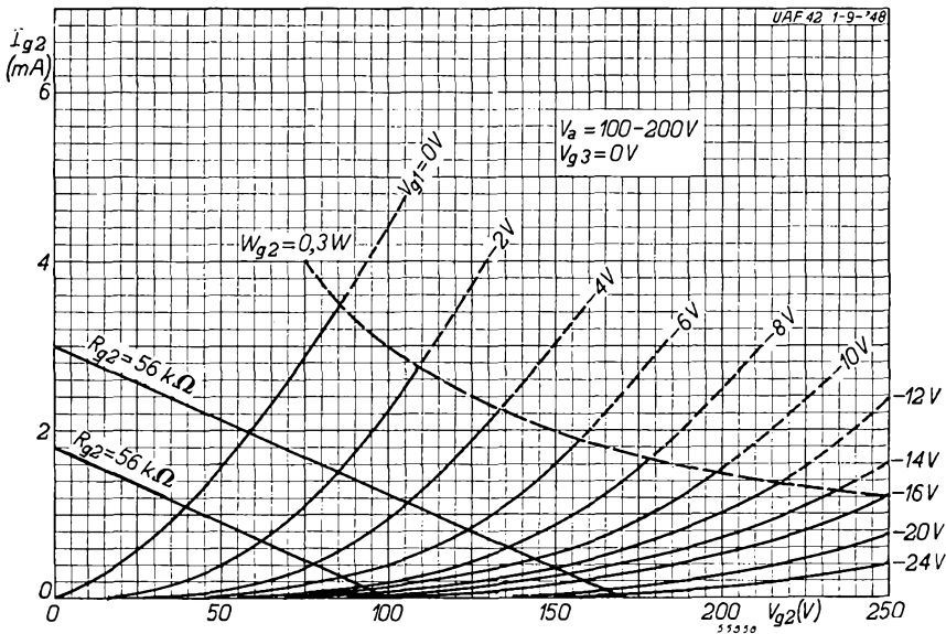
Fig. 14 Screen grid current ( I_{g2} ) of the pentode section of the UAF 42 as a function of the screen grid voltage ( V_{g2} ) with grid bias ( V_{g1} ) as parameter. The maximum permissible screen grid dissipation (0.3 W) is indicated by the dotted line. The straight lines give the working characteristic for a screen grid series resistor of 56 k \Omega , at supply voltages of 170 and 100 V.
