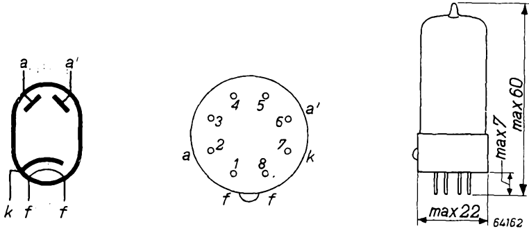
Fig. 2 Electrode arrangement, electrode connections and dimensions in mm of the EZ 41.
