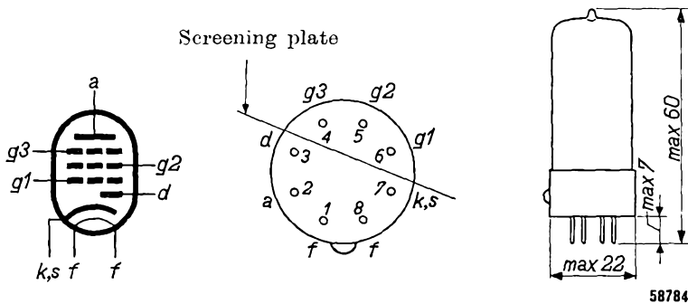
Fig. 8 Electrode arrangement, electrode connections and maximum dimensions in mm of the EAF 42. The screening plate shown in the centre diagram serves to reduce unwanted coupling in the wiring.
