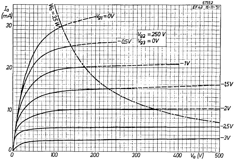
Fig. 5 I_a/V_a characteristics of the EF 42. The broken line indicates the maximum permissible anode dissipation ( P_a = 3.5 W ).
