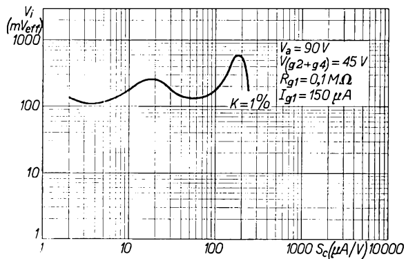
Fig. 17 The voltage ( V_i ) of an interfering signal at the control grid producing 1% cross-modulation is shown as a function of the conversion conductance.
