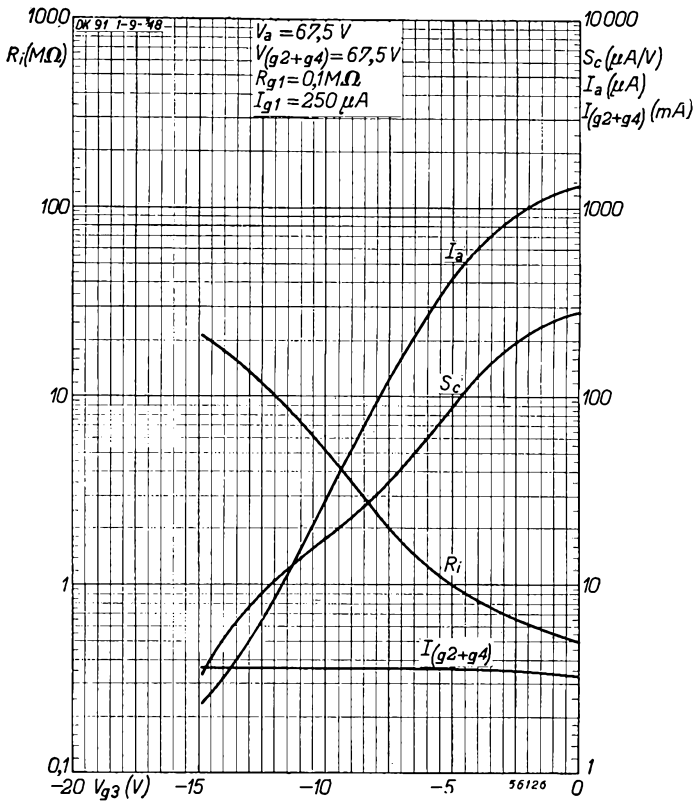
Fig. 15 As Figs. 13 and 14, at V_a = V_{g_2+g_4} = 67.5 \text{ V} .
