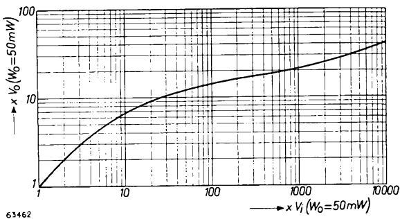
Fig. 2. A.G.C. curve of the receiver.
