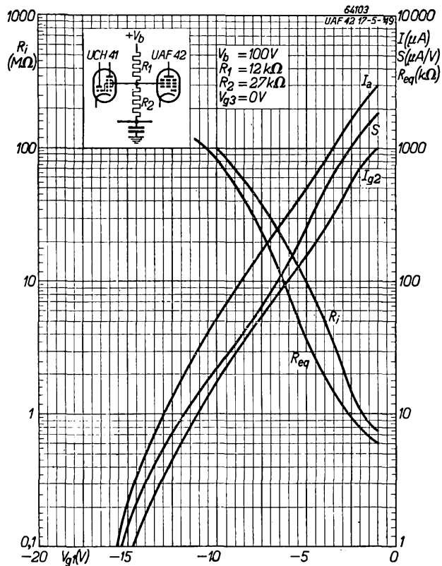
Fig. 15 As Figs. 10 and 11, but with the screen grid voltage of the UAF 42 obtained by means of the same potentiometer as that of the frequency changer UCH 41.
