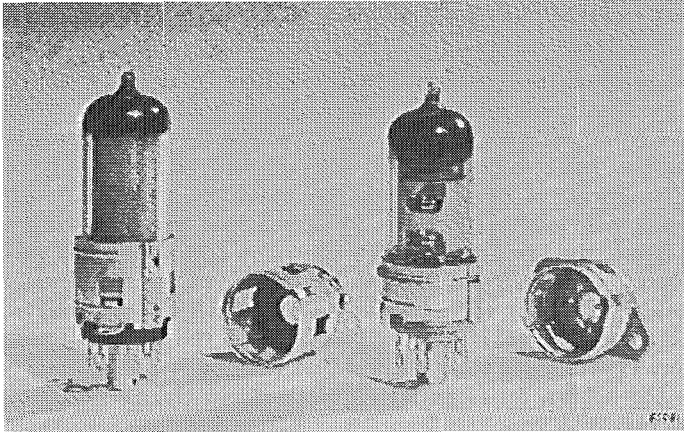
Fig. 6. Rimlock valveholders.
