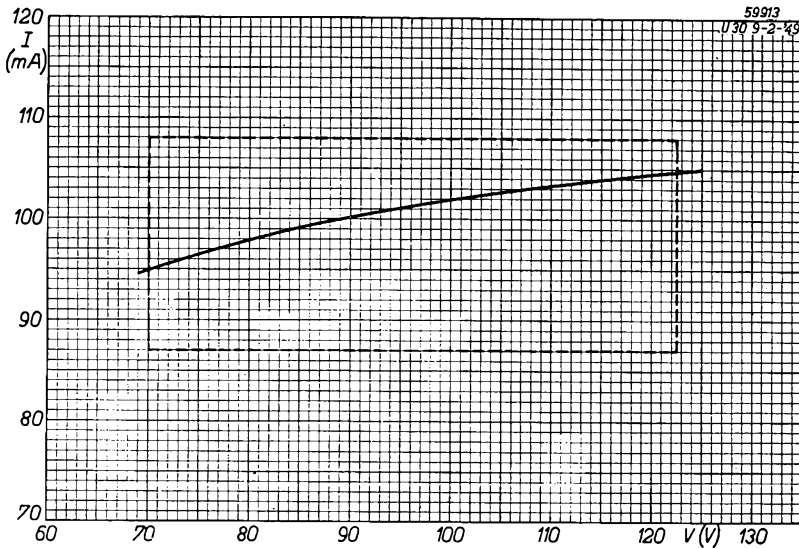
Fig. 3 Control characteristic of the U 30, current I flowing through the resistance wire as a function of the applied voltage V .
