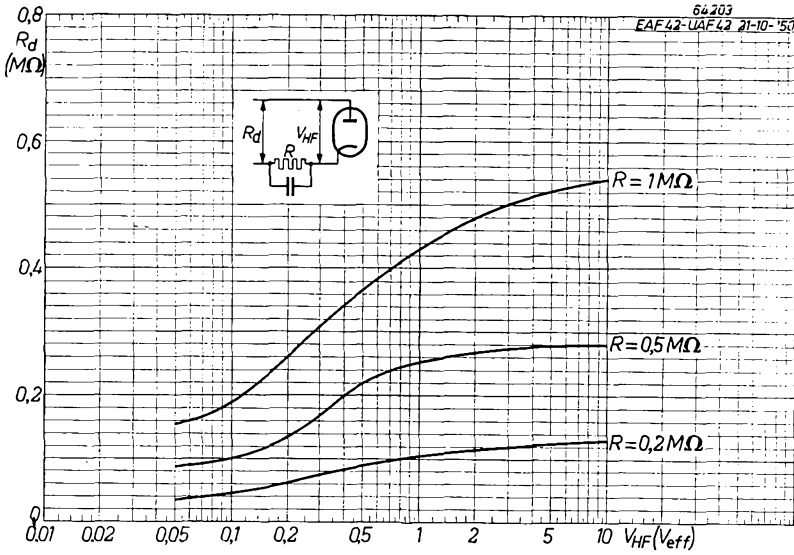
Fig. 13 Damping resistance of the diode of the UAF 42 as a function of the applied R.F. signal, for different values of the series resistor in the detector circuit. For detection characteristic of the diode see Fig. 7 in the description of the EBC 41.
