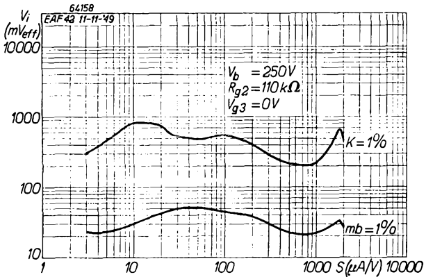
Fig. 15 R.M.S. voltage ( V_i ) of an interfering signal at the grid of the EAF 42, producing 1% cross modulation (curve K = 1\% ), together with the R.M.S. value ( V_i ) of a hum voltage at the grid, resulting in 1% modulation hum (curve m_b = 1\% ), measured as a function of the mutual conductance in the I.F. circuit shown in Fig. 2.
