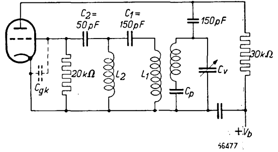
Fig. 4 Oscillator circuit for short waves. An extra coil, L_2 , is introduced between grid capacitor and feedback coil, thus increasing the oscillator voltage at the upper end of the wave-band.
