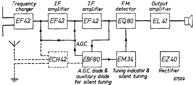
Fig. 1a. Block diagram of the F.M. section.
