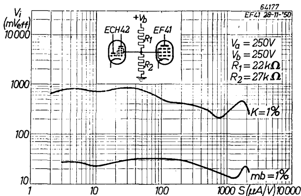
Fig. 9. As Fig. 8, with the screen grid voltage of the EF 41 and that of the ECH 42 applied by means of the same potentiometer.
