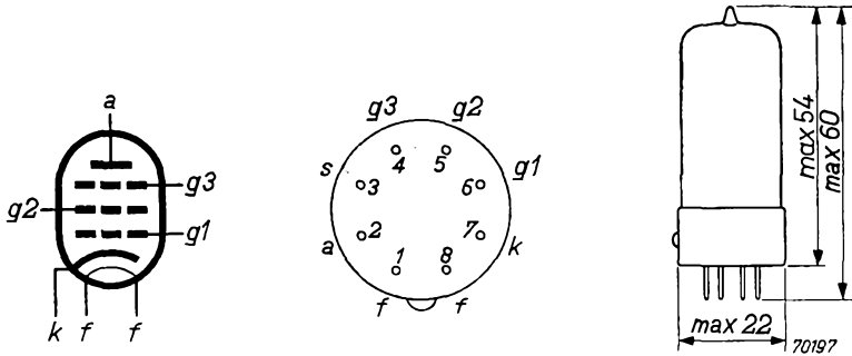
Fig. 1 Electrode arrangement, electrode connections and dimensions in mm of the UF 42.
