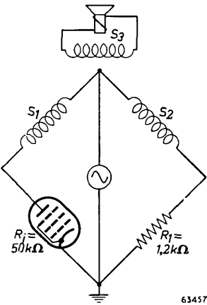
Fig. 7. Equivalent diagram of the hum-compensation circuit.
