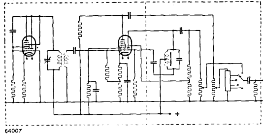
Skeleton circuit of the GM 2884.
