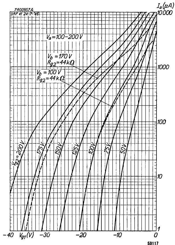
Fig. 6 Anode current ( I_a , Fig. 6) and mutual conductance ( S , Fig. 7) of the UAF 41 as functions of the grid bias V_{g1} for different values of the screen grid voltage ( V_{g2} ). The dotted lines indicate the variations in anode current and mutual conductance when a series resistor R_{g2} of 44 k \Omega is included in the screen grid circuit.
