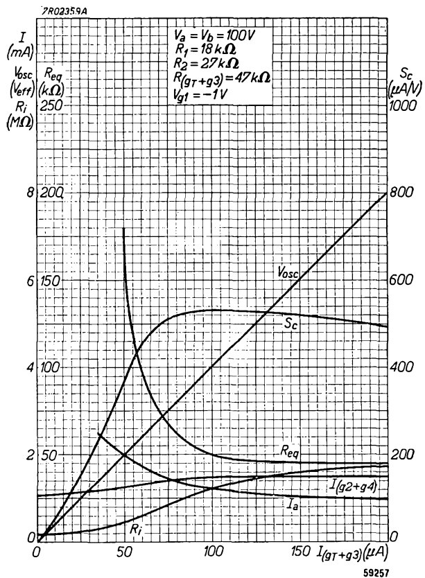
Fig. 14 As Figs. 12 and 13, but for grid leak R_{gT+g3} of 47 kΩ.
