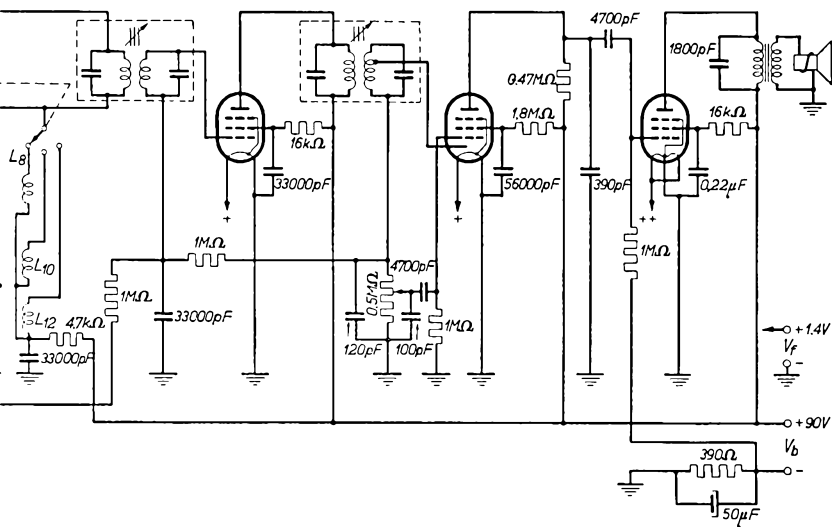
Fig. 1 4-valve battery receiver.
