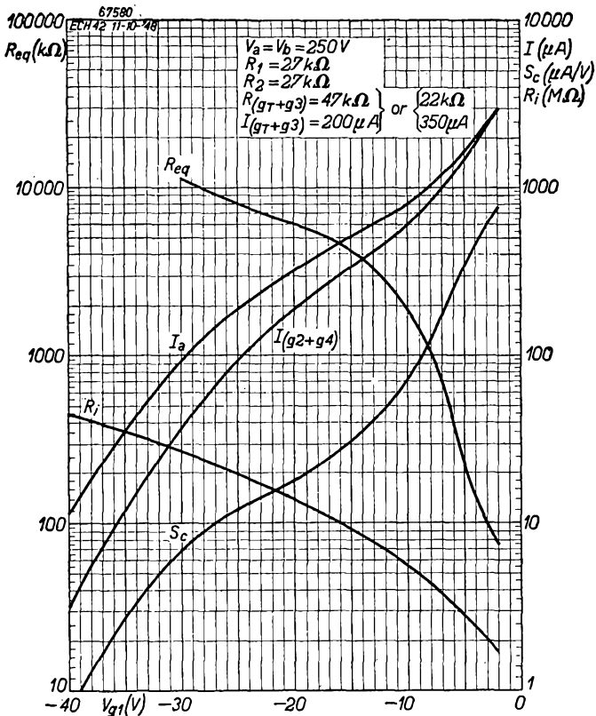
Fig. 8 Anode current ( I_a ), screen grid current ( I_{g_2+g_4} ), conversion conductance ( S_c ), internal resistance ( R_i ) and equivalent noise resistance ( R_{eq} ) as functions of the grid bias ( V_{g1} ). Measured in the circuit shown in Fig. 3.
