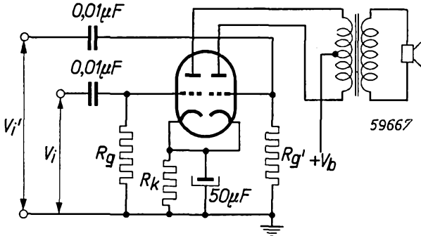
Fig. 5 The ECC 40 used as a push-pull output valve.
