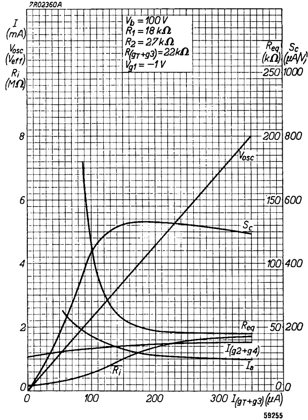
Fig. 12 Anode current ( I_a ), conversion conductance ( S_c ), oscillator voltage ( V_{osc} ), internal resistance ( R_i ) and equivalent noise resistance ( R_{eq} ) of the UCH 42 as functions of the oscillator grid current ( I_{gT+g3} ) for a grid leak R_{gT+g3} of 22 k \Omega . Measured in the circuit shown in Fig. 3. Fig. 12 : supply voltage V_b = 100\text{ V} ; Fig. 13 : V_b = 170\text{ V} .
