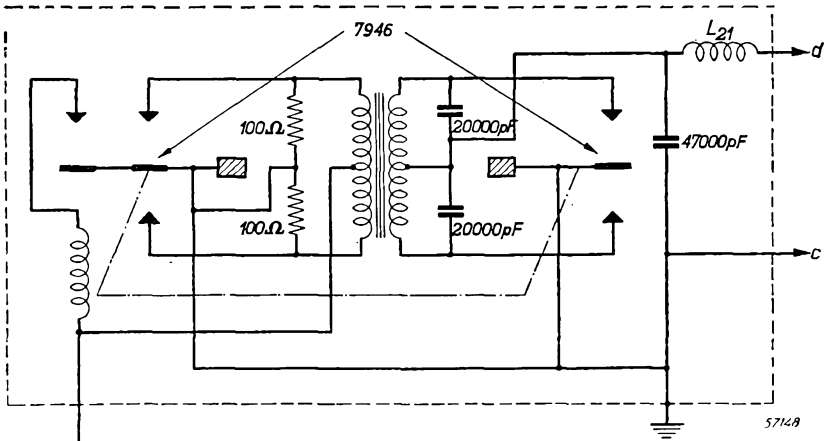
Fig. 7 Circuit of the vibrator section based on a synchronized vibrator
