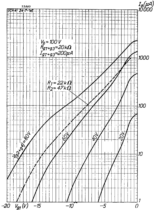
Fig. 6 Anode current ( I_a ) of the UCH 41, measured on oscillating valve, as a function of the grid bias ( V_{g1} ) with screen grid voltage ( V_{g2+g3} ) as parameter. The dotted curves represent the anode current when the screen grid voltage is derived from a potentiometer ( R_1 , R_2 , see Fig. 3). Fig. 6: supply voltage V_b = 100 \text{ V} ; Fig. 7: V_b = 170 \text{ V} .
