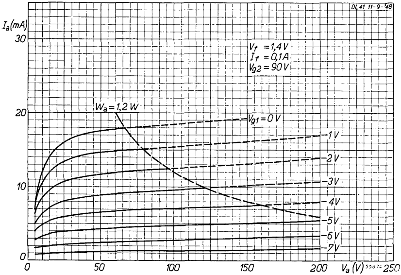
Fig. 9 I_a/V_a characteristics for a screen grid voltage of 90 V. Filament connections 1 and 7+8 ( V_f=1.4 V, I_f=100 mA).
