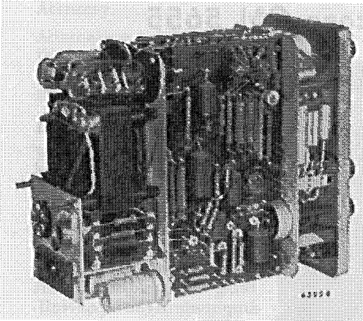
Interior view of the GM 5655; note the very compact, but readily accessible, arrangement.
