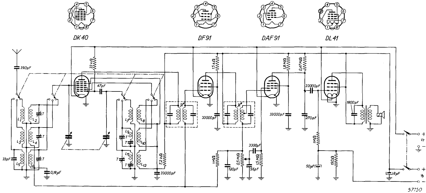
Fig. 1. A 4-valve battery receiver.
