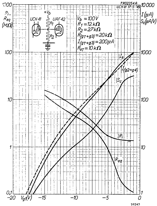
Fig. 19 As Fig. 10 and Fig. 11, but with the screen grids of the UCH 41, together with that of the UAF 42, fed by means of a common potentiometer. Measurements taken in the circuit shown in Fig. 5. Fig. 19: supply voltage V_b = 100V ; Fig. 20: V_b = 170V .
