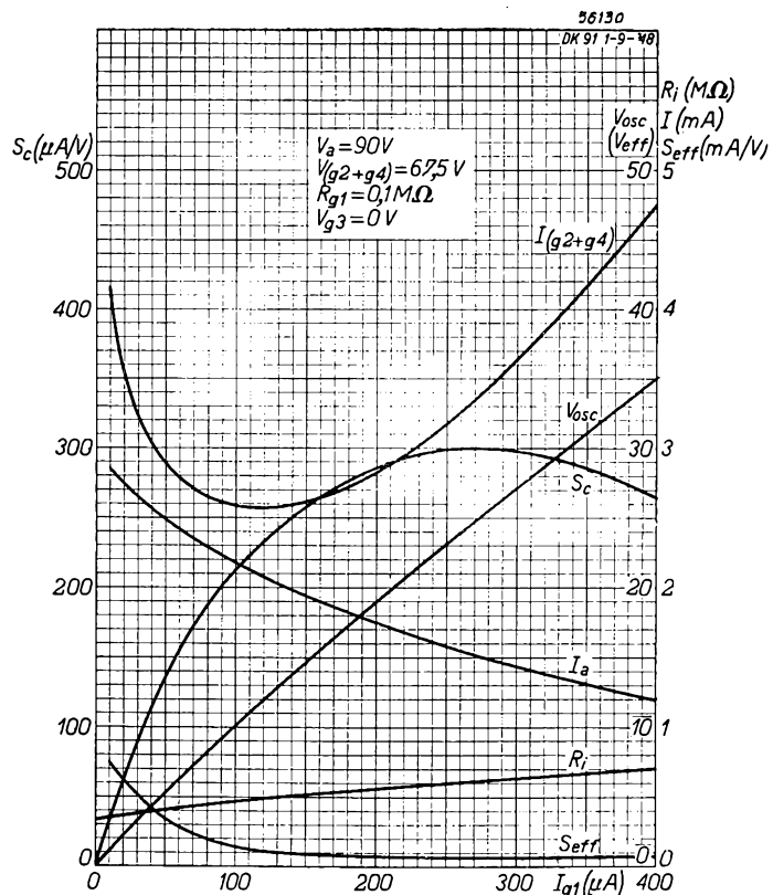
Fig. 12 As Figs. 9 and 10, at V_a = 90 \text{ V} and V_{g2+g1} = 67.5 \text{ V} .
