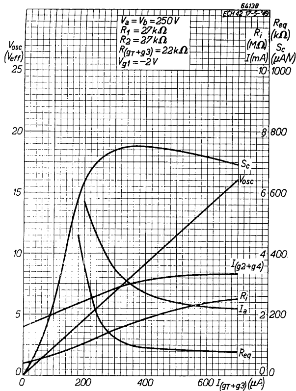
Fig. 10 Anode current ( I_a ), screen grid current ( I_{g_2+g_4} ), oscillator voltage ( V_{osc} ), conversion conductance ( S_c ), internal resistance ( R_i ) and equivalent noise resistance ( R_{eq} ) as functions of the oscillator grid current.
