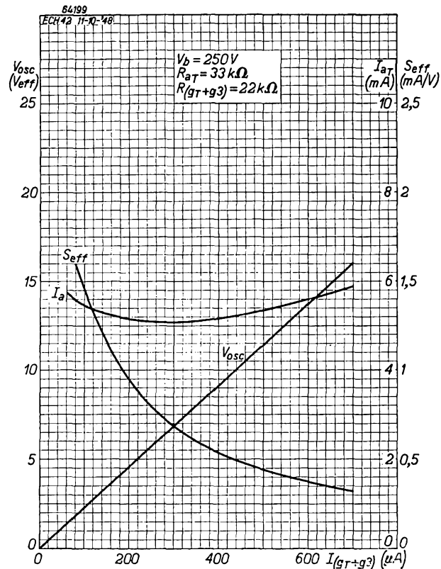
Fig. 12 Triode system: anode current ( I_{aT} ), oscillator voltage ( V_{osc} ) and effective slope ( S_{eff} ) as functions of the oscillator grid current ( I_{gT+g3} ).
