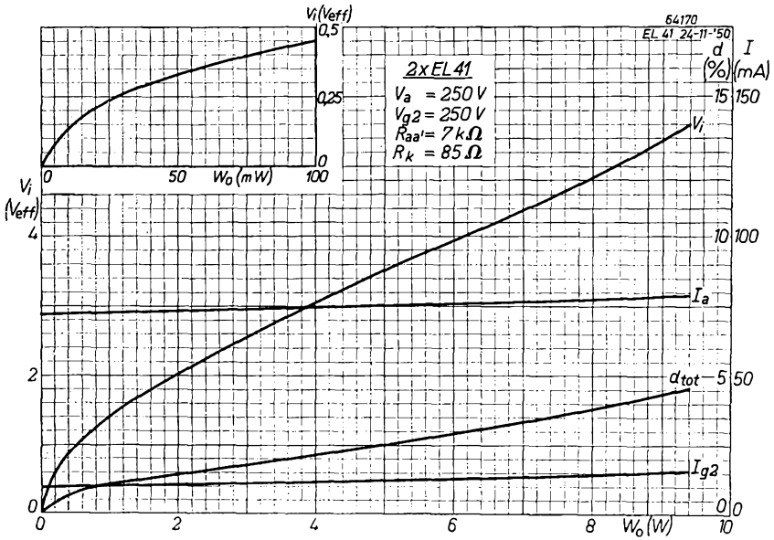
Fig. 8 As Fig. 7, for two EL 41 valves in Class A push-pull. I_a =total anode current, I_{g2} =total screen grid current, V_i =A.C. input voltage.
