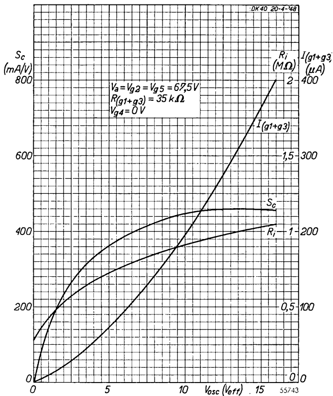
Fig. 14 Conversion conductance ( S_c ), internal resistance ( R_i ) and oscillator current ( I_{g1+g3} ) as functions of the oscillator voltage ( V_{osc} ). Fig. 14: battery voltage 67.5 V.
