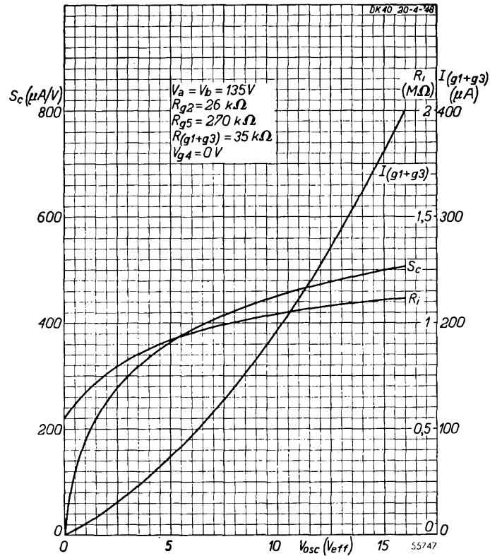
Fig. 17 As Fig. 14, but with 135 V battery.
