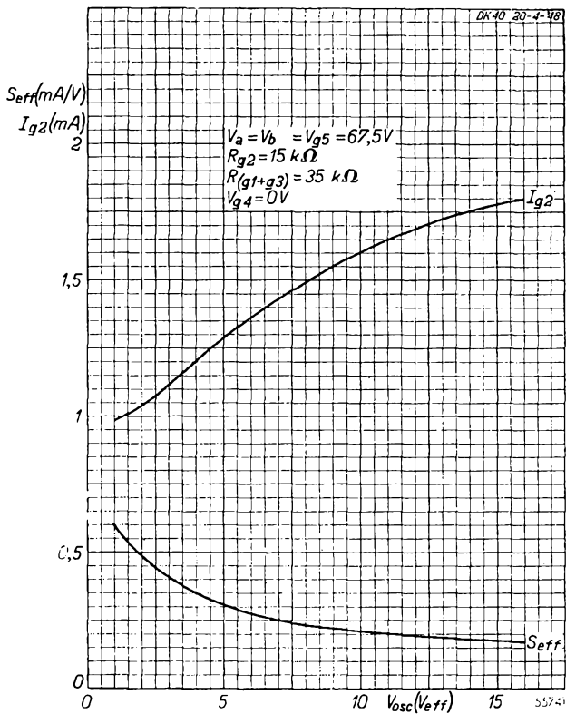
Fig. 20 As Fig. 19, but for the economy circuit (oscillator anode voltage V_{g2} = 45 V ).
