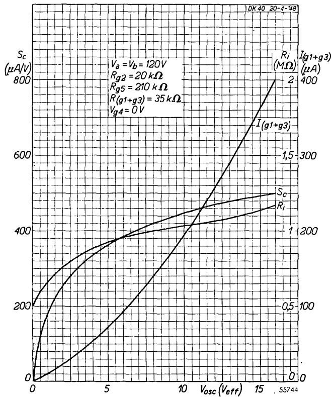
Fig. 16 As Fig. 14, but with 120 V battery.
