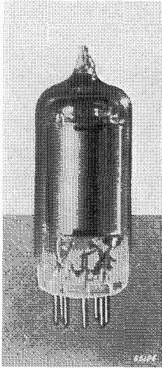
Fig. 1 The DF 91 (approximately full size).
