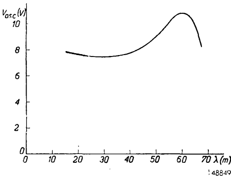
Fig. 5 Variations in the oscillator voltage as a function of the wavelength, relative to the circuit shown in Fig. 4.
