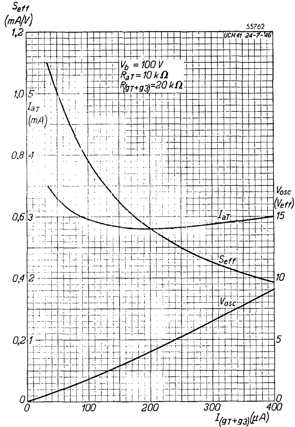
Fig. 17 Anode current ( I_a ), oscillator voltage ( V_{osc} ) and effective slope ( S_{eff} ) of the triode system of the UCH 41, as functions of the oscillator grid current ( I_{gT+g3} ). Fig. 17 : supply voltage V_b = 100 \text{ V} ; Fig. 18 : V_b = 170 \text{ V} .
