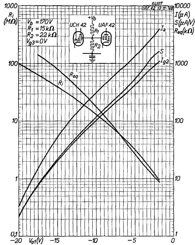
Fig. 19 As Figs. 10 and 11, but with the screen grid feeds of the UAF 42 and UCH 42 taken from a common potentiometer.
