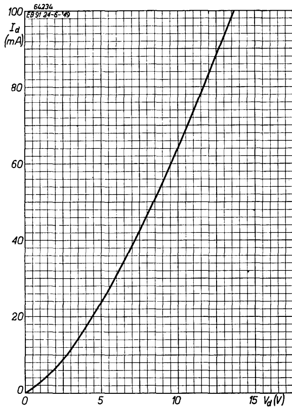
Fig. 4 The current I_d of each system of the EB 41, as a function of the voltage V_d .
