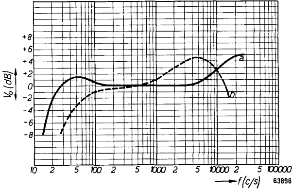
Fig. 3. Response characteristic of the A.F. section with the volume control at: a. 1/10 of its total resistance, b. maximum setting.
