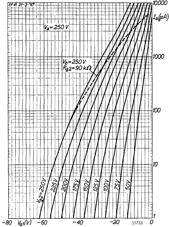
Fig. 4 Anode current I_a (Fig. 4) and slope S (Fig. 5) as functions of the grid bias V_{g1} for various values of the screen grid voltage V_{g2} . The dotted lines indicate the I_a (Fig. 4) and S (Fig. 5) when the screen grid feed is applied through a series resistor R_{g2} of 90\text{ k}\Omega .
