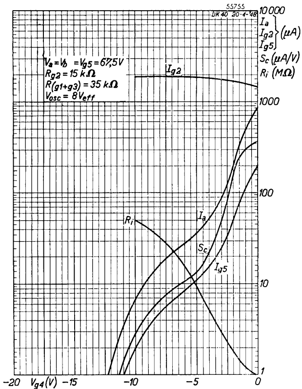
Fig. 10 As Fig. 6, but for the economy circuit (oscillator anode voltage V_{g2} = 45 V ).
