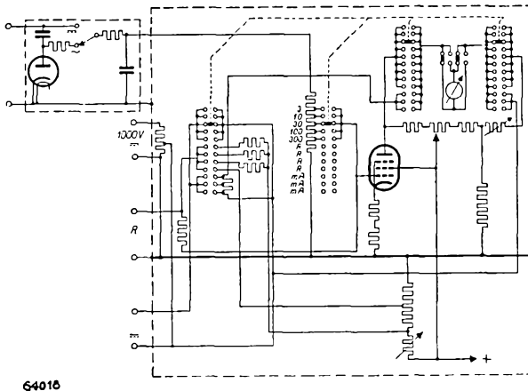
Skeleton circuit of the GM 7635.
