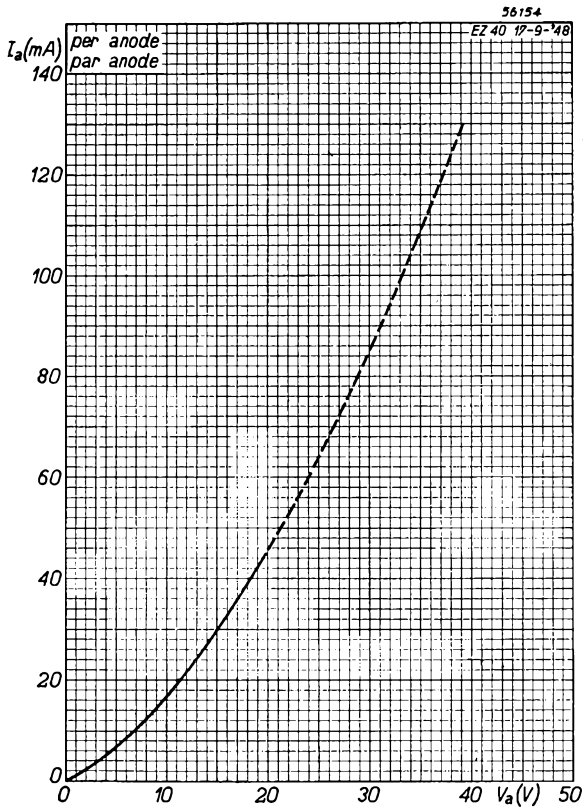
Fig. 3 Anode current ( I_a ) of the EZ 40 as a function of the applied D.C. voltage ( V_a ); since the maximum permissible current per anode is 45 mA, the curve above this value is drawn as a dotted line.
