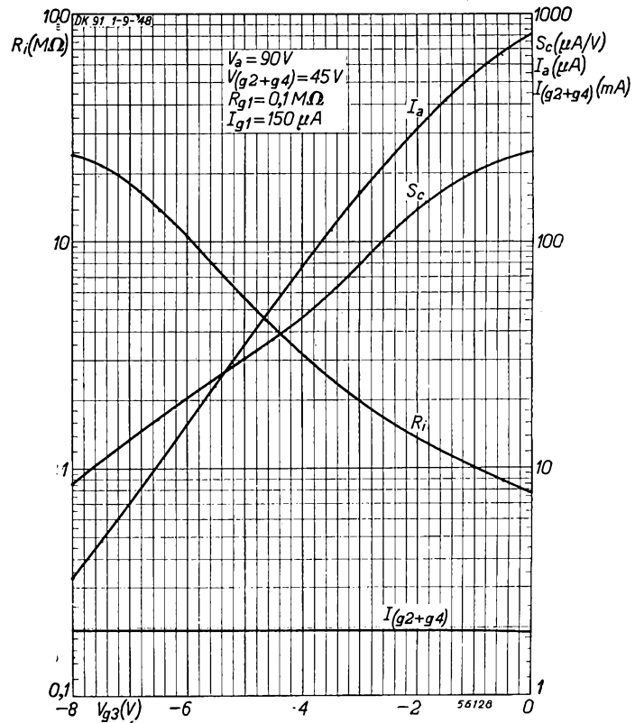
Fig. 13 Anode current ( I_a ), screen grid current ( I_{g2+g4} ), conversion conductance ( S_c ) and internal resistance ( R_i ) as functions of the grid bias ( V_{g3} ). Measured on oscillating valve in circuit shown in Fig. 2.
