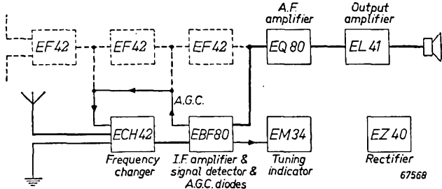
Fig. 1b. Block diagram of the A.M. section.
