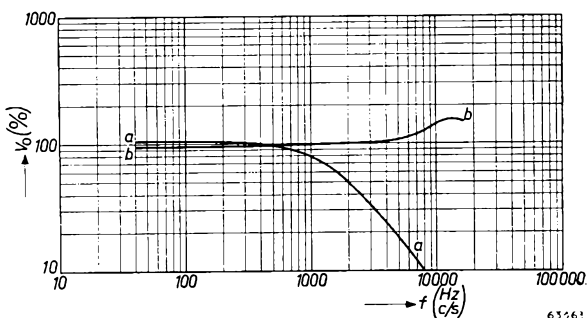
Fig. 3. Frequency-response characteristic a) with, and b) without tone control.
