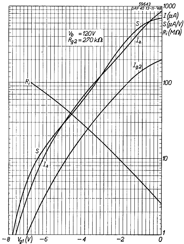
Fig. 7 As Fig. 6, but for a supply voltage of 120 V.
