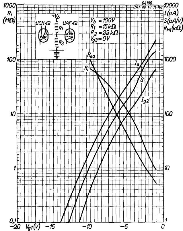
Fig. 19 As Figs. 10 and 11, but with the screen grid feeds of the UAF 42 and UCH 42 taken from a common potentiometer.
