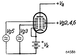
Fig. 2 Control and supply voltages for the EQ 80.
