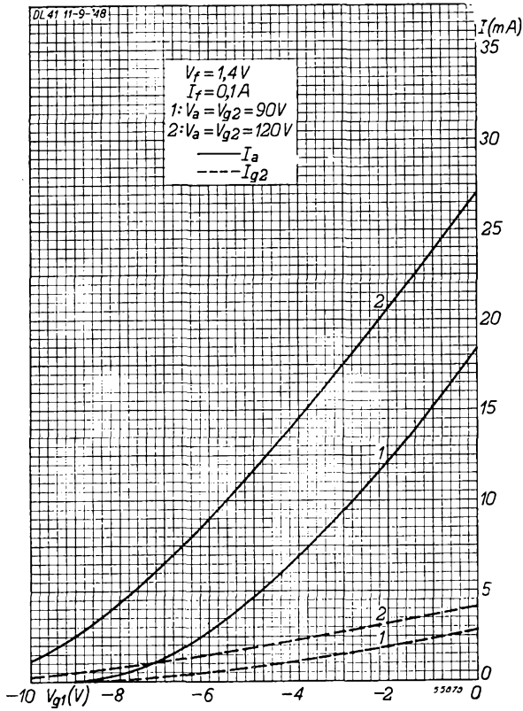
Fig. 8 Anode current ( I_a ) and screen grid current ( I_{g2} ) as functions of the grid bias ( V_{g1} ), with battery voltages of 90 and 120 V. Filament connections 1 and 7+8 ( V_f=1.4 V , I_f=0.1 A ).
