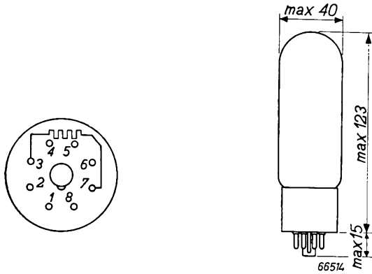
Fig. 2 Electrode connections and dimensions in mm of the U 30.
