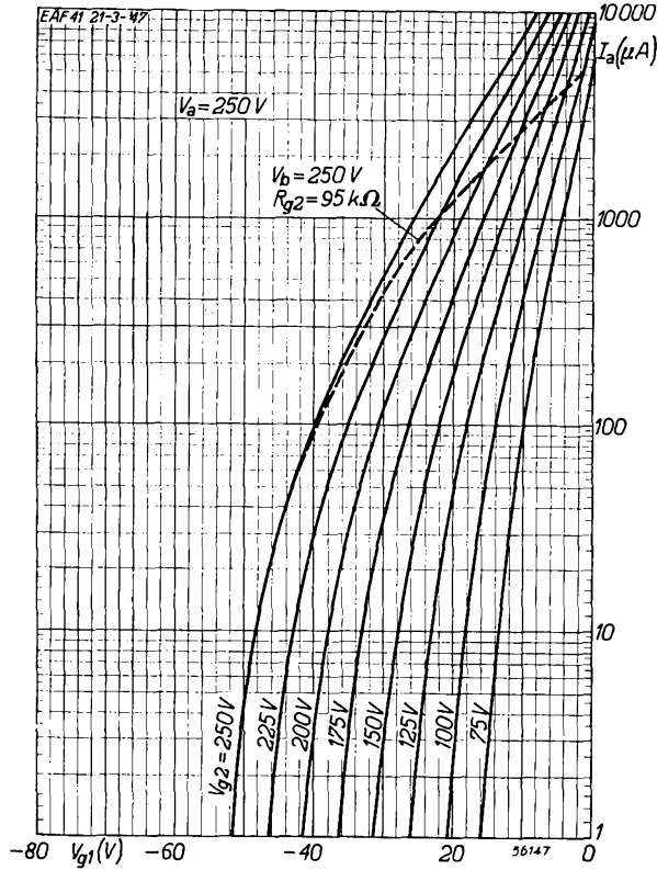
Fig. 10 Anode current (Fig. 10) and mutual conductance (Fig. 11) of the EAF 41 as functions of the grid bias for different screen grid voltages. The broken lines represent the anode current and slope with a 95 k \Omega -resistor in series with the screen grid.
