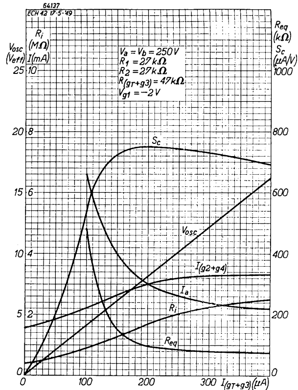
Fig. 10 Anode current ( I_a ), screen grid current ( I_{g_2+g_4} ), oscillator voltage ( V_{osc} ), conversion conductance ( S_c ), internal resistance ( R_i ) and equivalent noise resistance ( R_{eq} ) as functions of the oscillator grid current.
