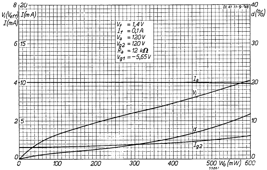
Fig. 12 As Fig. 10, but for a 120 V battery. Filament connections 1 and 7+8 ( V_f=1.4 V , I_f=100 mA ).
