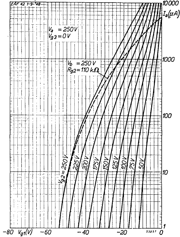
Fig. 12 Anode current (Fig. 12) and mutual conductance (Fig. 13) of the EAF 42 as functions of the grid bias for various screen grid voltages. The broken lines represent the anode current and slope of the I.F. valve EAF 42 in the circuit of Fig. 2.
