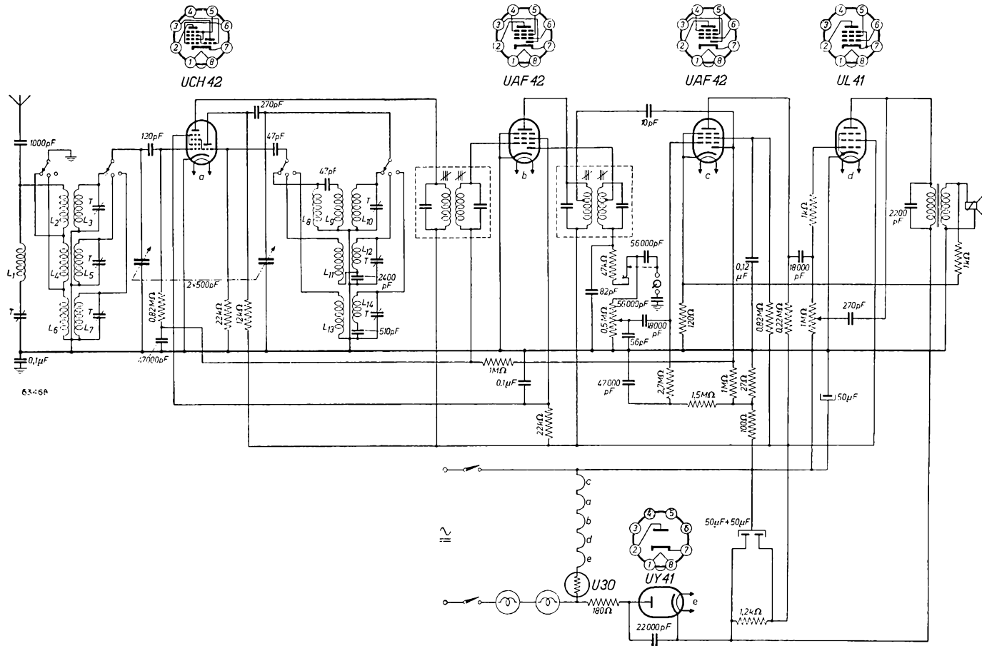
Fig. 1. Circuit of 5-valve A.C./D.C. receiver with barretter.
