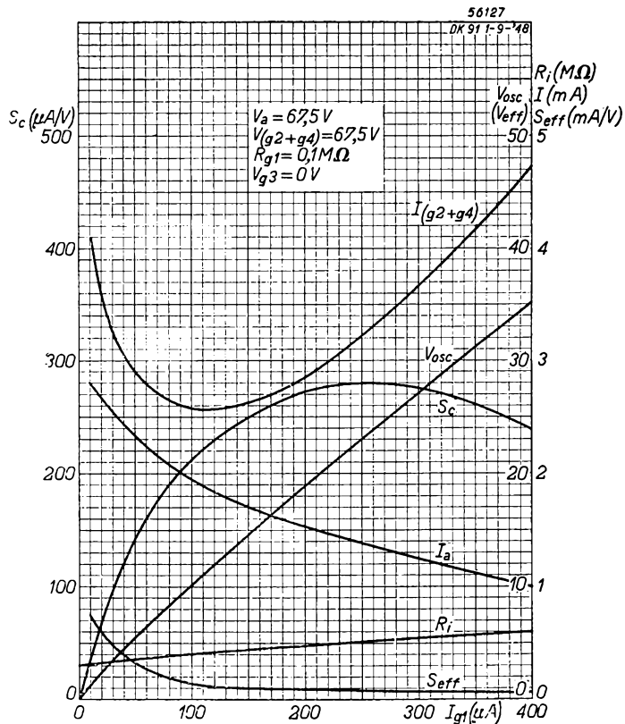
Fig. 11 As Figs. 9 and 10, but at V_a = V_{g2+g4} = 67.5 \text{ V} .
