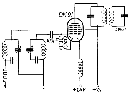
Fig. 6 Mixer circuit employing the DK 91 with the filament connected to a tapping on the oscillator coil.
