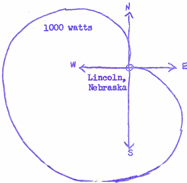
DAY PATTERN: 2 tower cardioid, null protecting northeast
