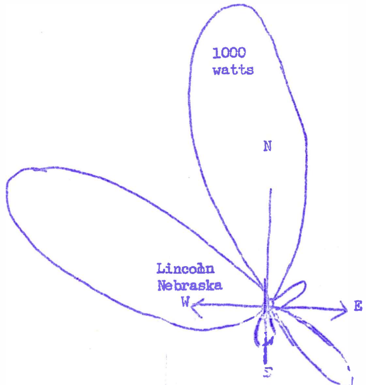
NIGHT PATTERN: 4 towers with lobes north, northwest, west-southwest, south-southeast
