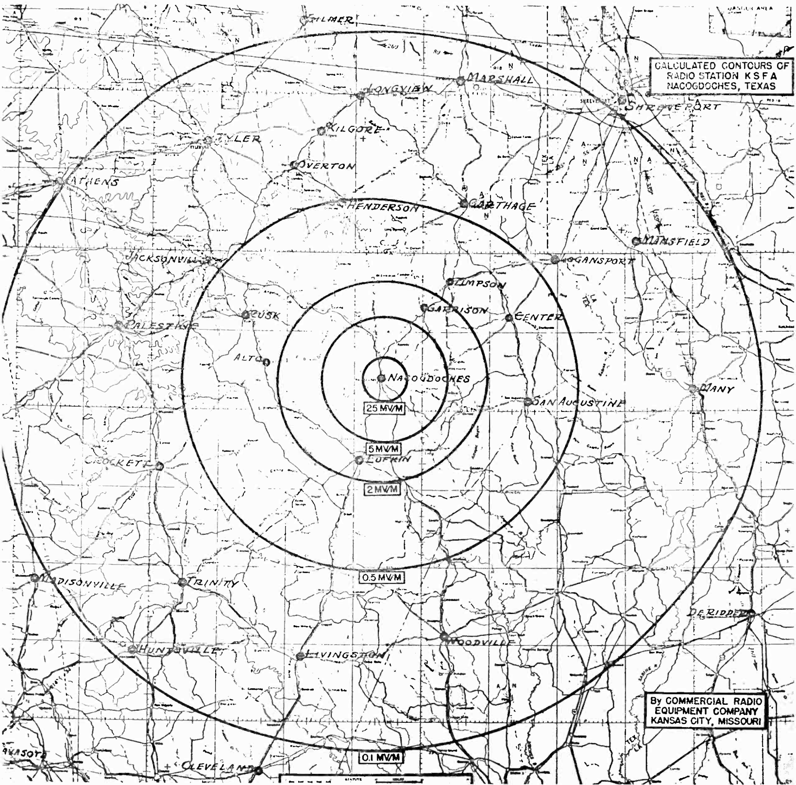
Estimated Coverage Map - Station KSFA - East Texas
