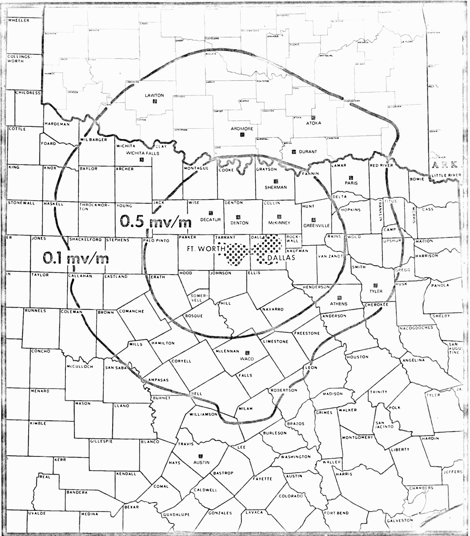
KNOK-AM COVERAGE MAP 970 kc. 1,000 watts
