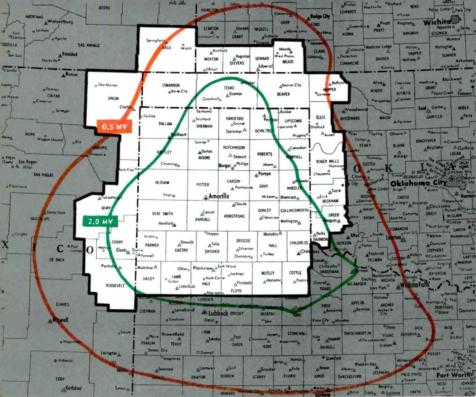
KGNC AM COVERAGE
