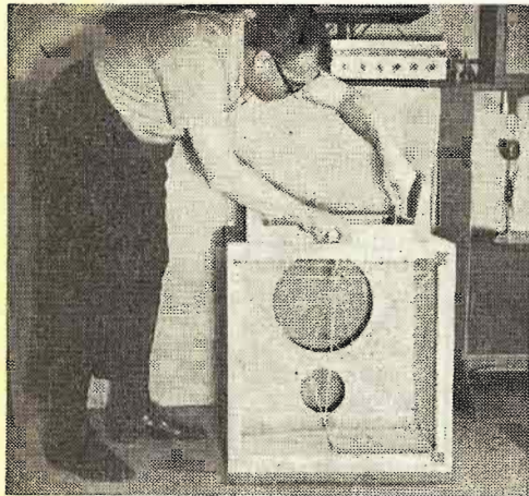
At right base is being attached to bottom of cabinet. Note strings holding the unit together while glue sets. Above, speaker and acoustical material in place—now screw back on.
